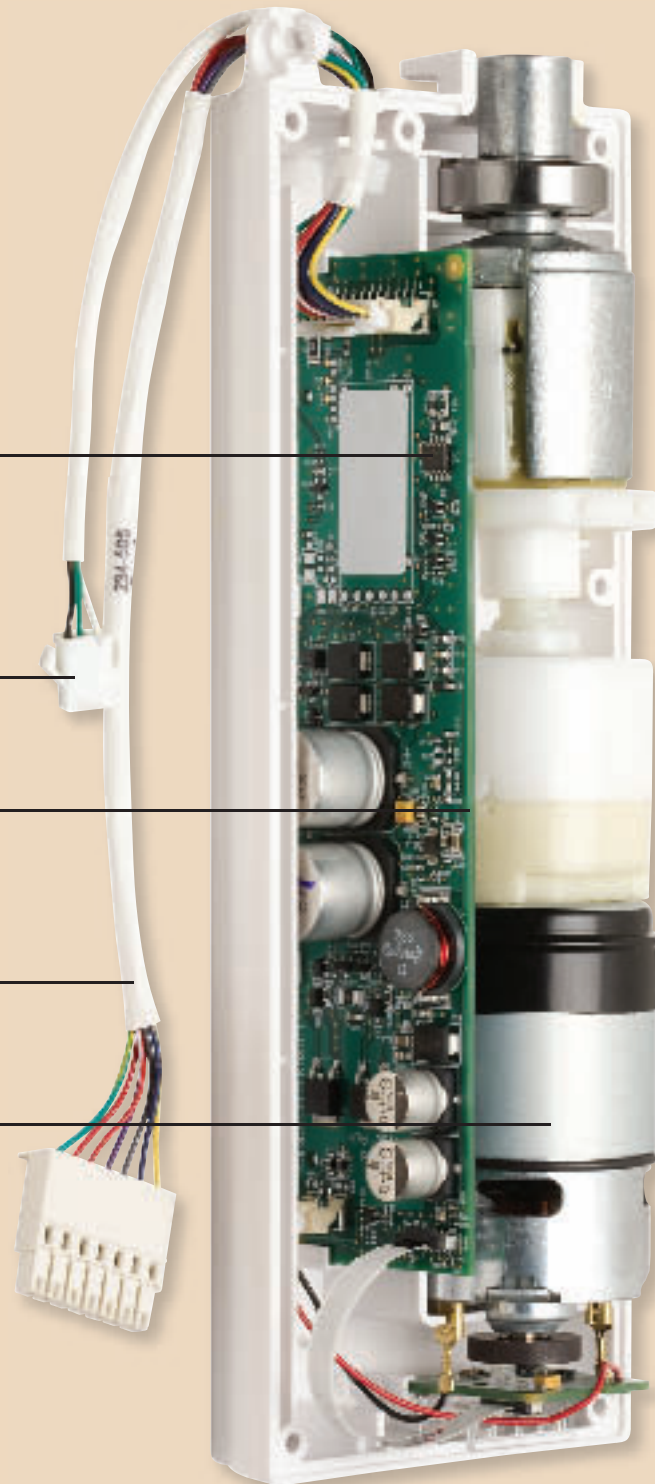
Lutron® drapery drive with cover removed
