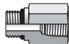
Conversion Adapter SAE-ORB / METRIC (F5OHG8)
