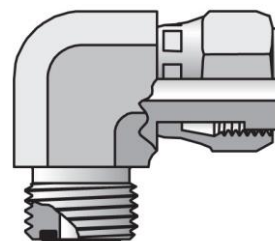
SWIVEL NUT ELBOW ORFS / ORFS (C6LO-S)
