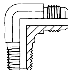
90° MALE ELBOW 2103 (CTX)
