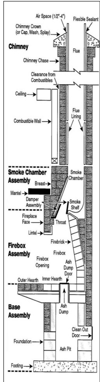
Parts of a masonry fireplace
