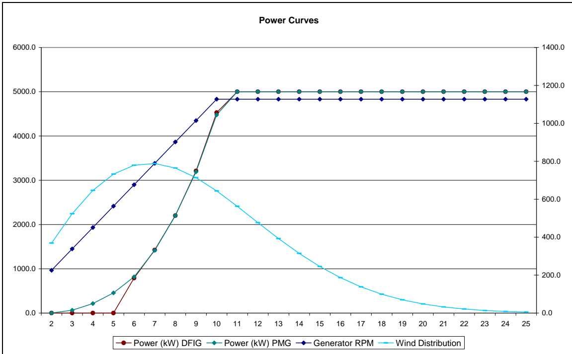
Figure 9: DFIG vs. PMG Power Curves with Wind Distribution
