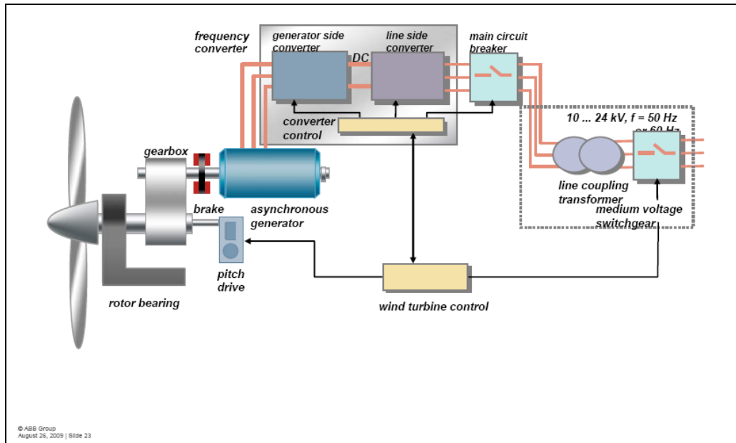
Figure 3: Layout of Permanent Magnet Generator based power system, courtesy ABB
