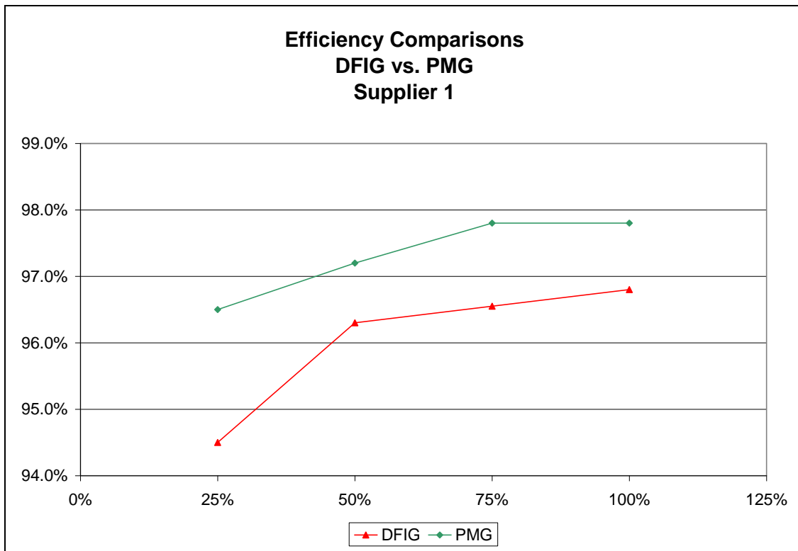
Figure 6: DFIG vs. PMG Efficiency Supplier 1
