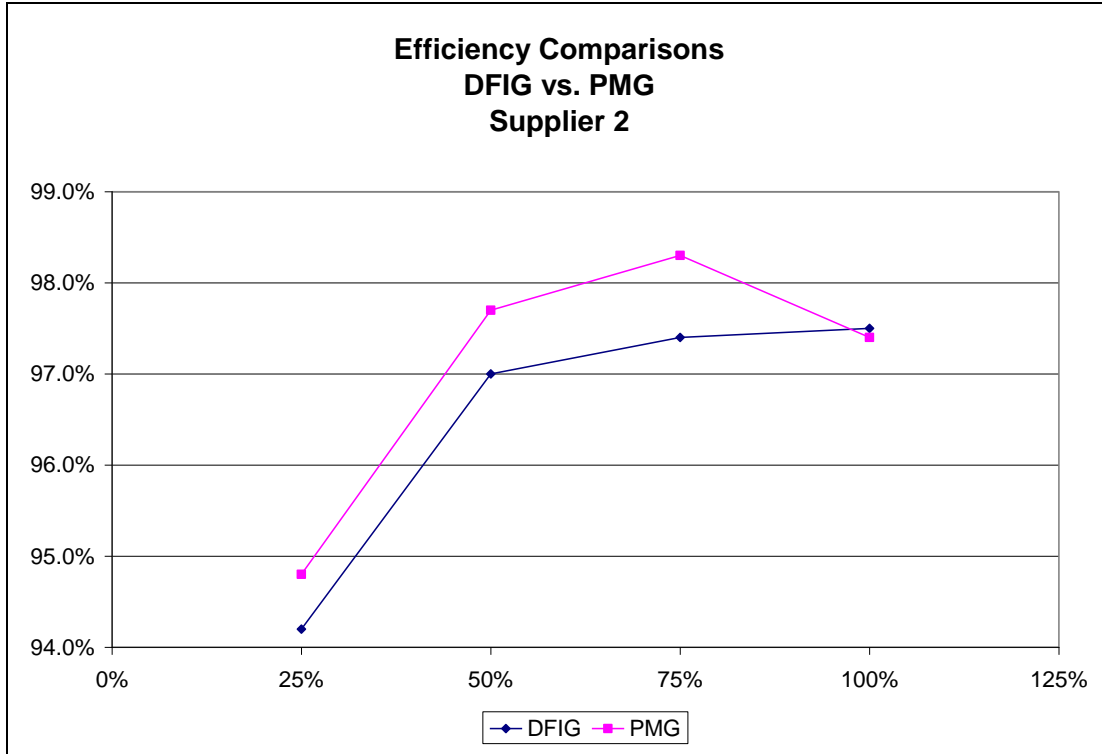
Figure 7: DFIG vs. PMG Efficiency Supplier 2
