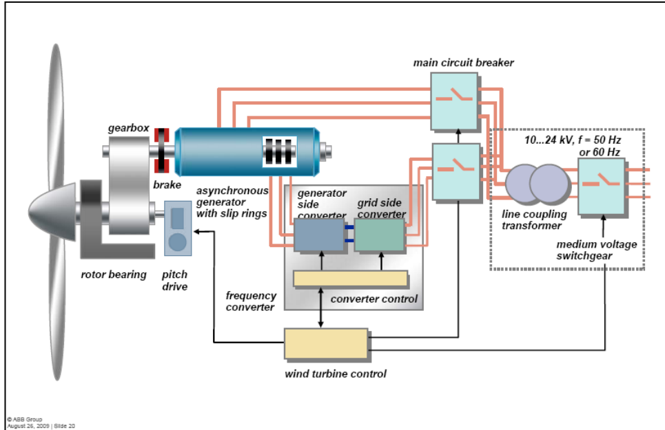
Figure 1: Layout of DFIG power system, courtesy ABB
