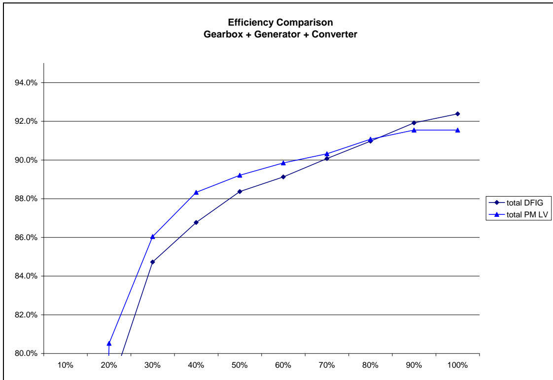
Figure 8: DFIG vs. PMG Aggregate Efficiency Curves
