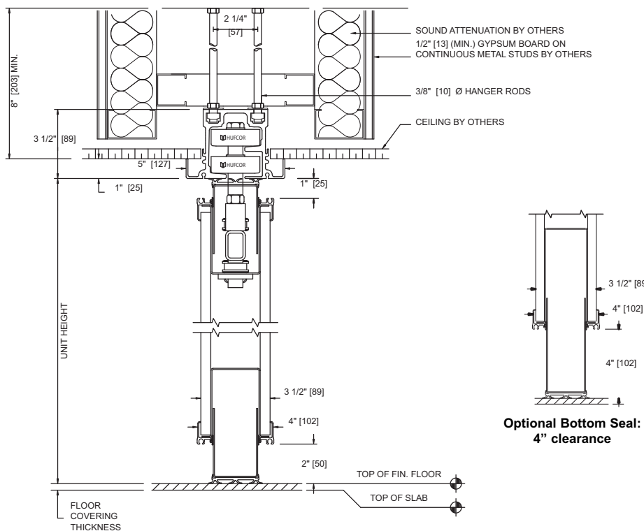
VERTICAL SECTION
