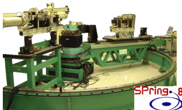
Spectrometer
