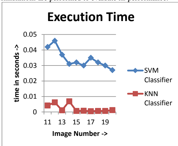
Fig.2: Execution Time
