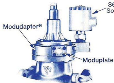
A4AS BACK PRESSURE REGULATOR WITH ELECTRIC SHUT-OFF VARIATION
