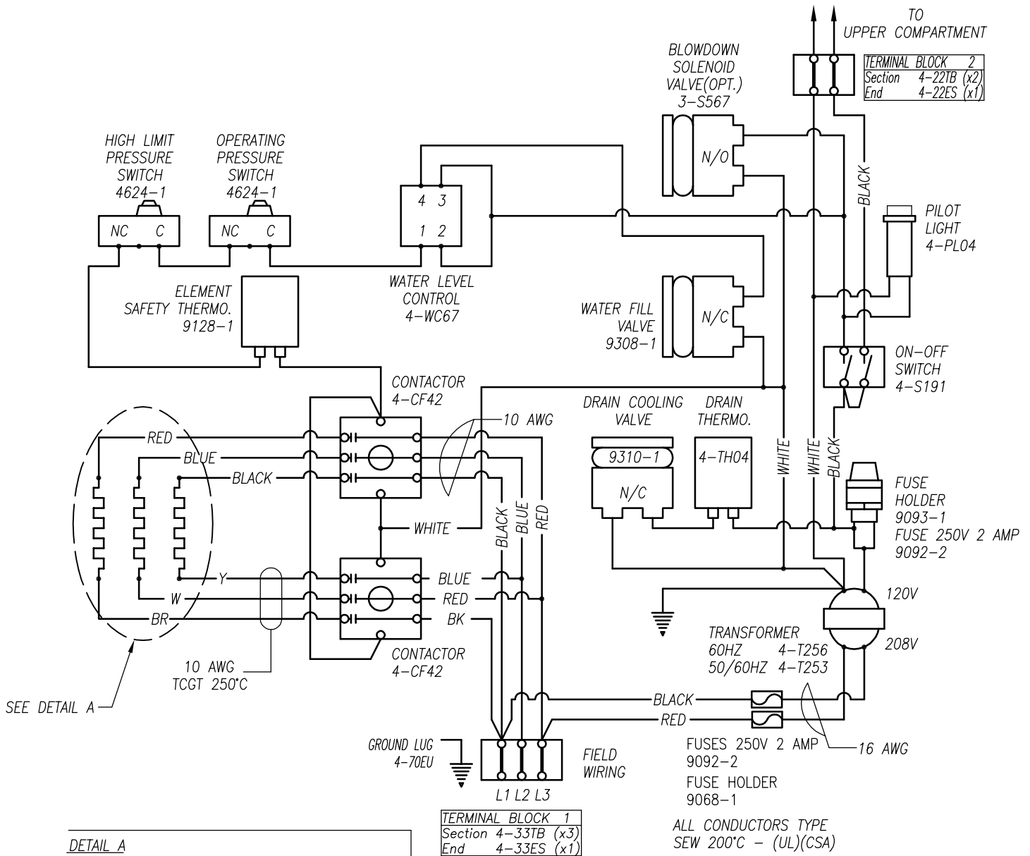
THREE PHASE CONNECTION
