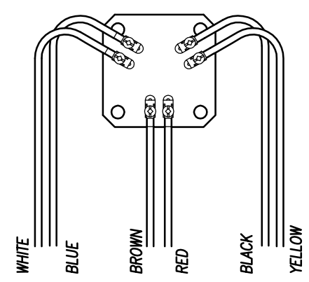
DETAIL A 7-5031 ELEMENT ASSY. THREE ELEMENTS @8000W 208V
