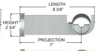
ACBRE-218-E 2 1/8" DIA EXTENDED SINGLE METAL BRACKET
