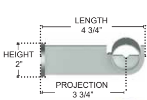
ACBRE-138-S 1 3/8" DIA STANDARD SINGLE METAL BRACKET
