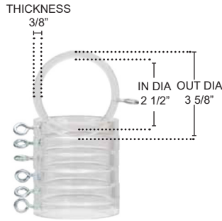
ACRS-218-7 ACRYLIC RING SET OF 7 for 2 1/8" Dia Pole
