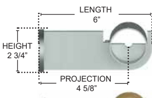
ACBRE-218-S 2 1/8" DIA STANDARD SINGLE METAL BRACKET
