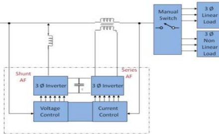
Fig.2: Dual UPQC.
