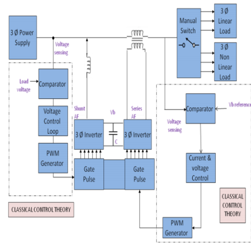
Fig.3: Control of iUPQC
