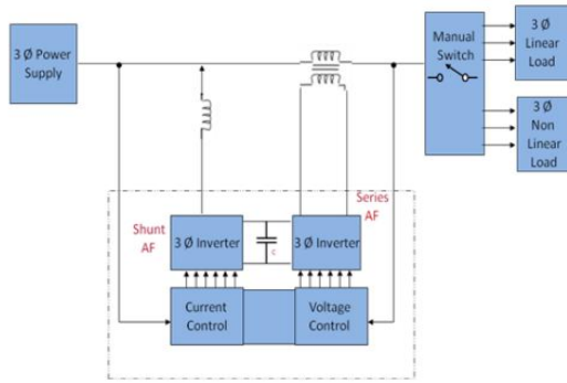
Fig.1: Convectional UPQC
