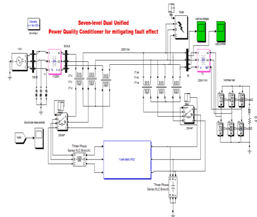
Fig.4: Simulation circuit diagram
