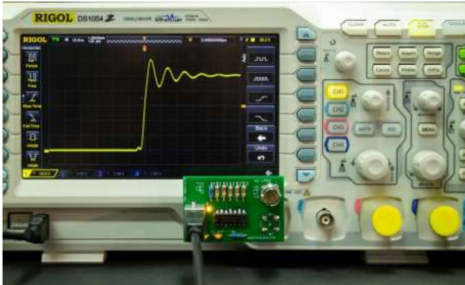
Image 2 - Close-Up of the board connected to CH. 1 of a DSO
