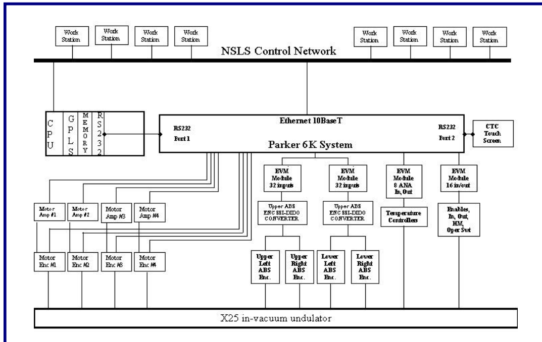
Figure 1: Integrated ADC Parker System with the NSLS Control System
