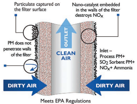
NO x and ammonia react with catalyst to destroy NO x .
