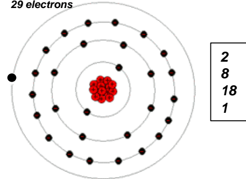
Copper Atom 29 electrons
