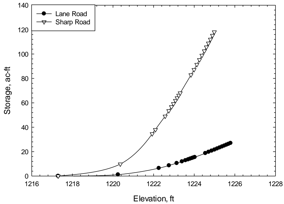
Fig. 13. Elevation vs. storage curves for the Lane Road Culvert and Sharp Road Culvert.
