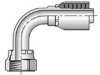
FLAT FACE FEMALE "SEAL LOK" SWIVEL 90° ELBOW LONG DROP 1J143
