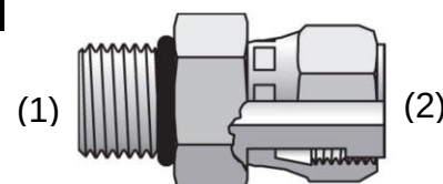
STRAIGHT THREAD SWIVEL CONNECTOR ORB / ORFS (F65OL)
