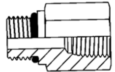
FEMALE PIPE ADAPTER 0502 (F5OG-S)
