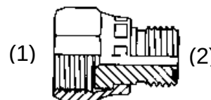
ORFS TUBE END REDUCER (TRLON-S)
