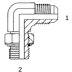
Male Elbow BSPP (C4OMXS)
