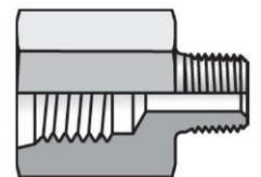
FEMALE STRAIGHT THREAD ADAPTER 0110 (FHG5-S)
