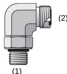
STRAIGHT THREAD ELBOW ORB / ORFS (C5OLO)
