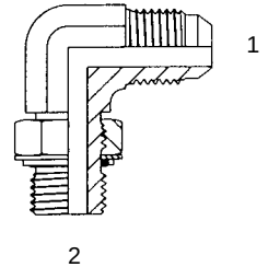
Male Elbow Metric Straight Thread (C8OMXS)
