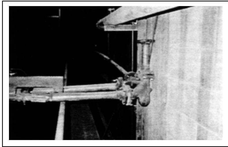
The solution to conveying system elbow wear at North Incinerator: the Smart Elbow™ in use in the lime injection conveying system.
