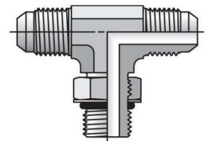
STRAIGHT THREAD BRANCH TEE 253T (S5OX)
