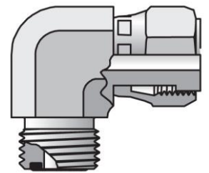
SWIVEL NUT ELBOW ORFS / ORFS (C6LO-S)
