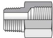
Conversion Adapter NPT-BSP (FHG4)
