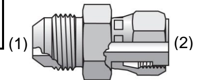
MALE SWIVEL ADAPTER JIC TUBE / ORFS SWIVEL (XHL6-S)
