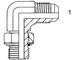
Male Elbow Metric Straight Thread (C8OMXS)
