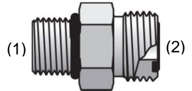
STRAIGHT THREAD CONNECTOR ORB / ORFS (F5OLO)
