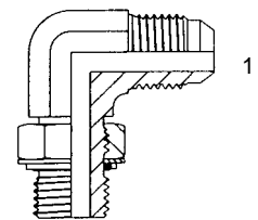
Male Elbow BSPP (C4OMXS)
