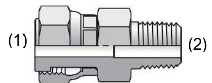
PIPE THREAD SWIVEL CONN ORFS SWIVEL / NPTF (F6L)
