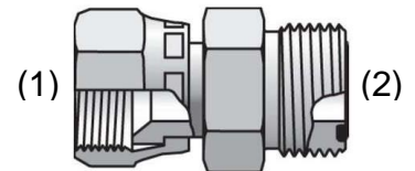
SWIVEL ADAPTER JIC TUBE SWIVEL / ORFS (LOHX6-S)
