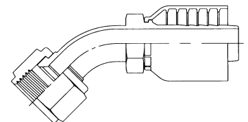
JIC 37° SWIVEL 45° ELBOW 13743
