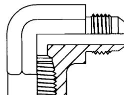
FEMALE 90° ELBOW 2203 (DTX)
