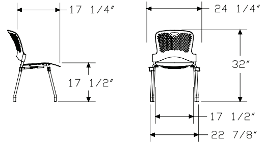
FLEXNET Seat
