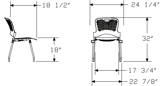
FLEXNET Seat
