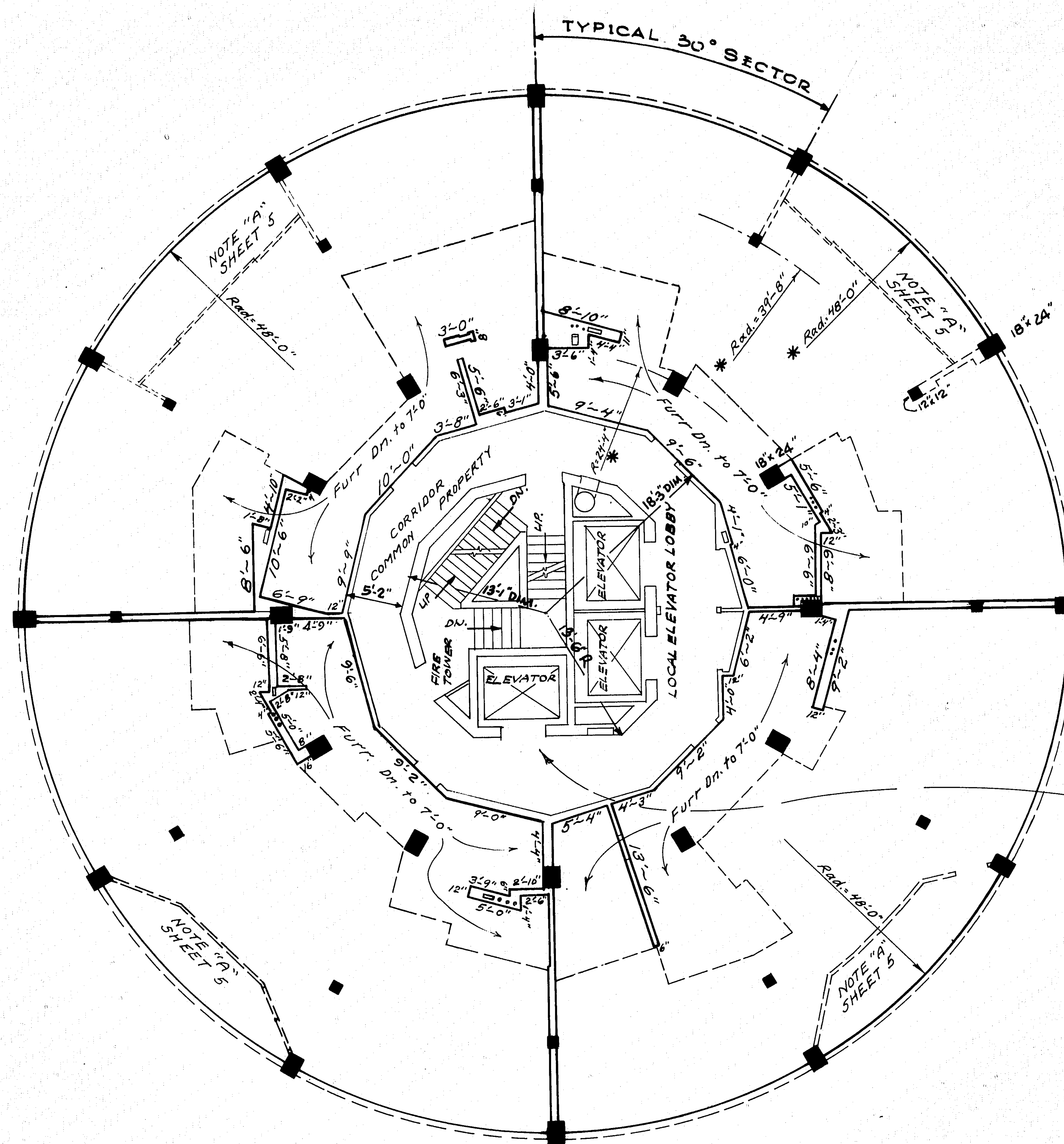
PLAN OF 28 TH FLOOR PENTHOUSES Scale - 1/8" = 1'-0"
