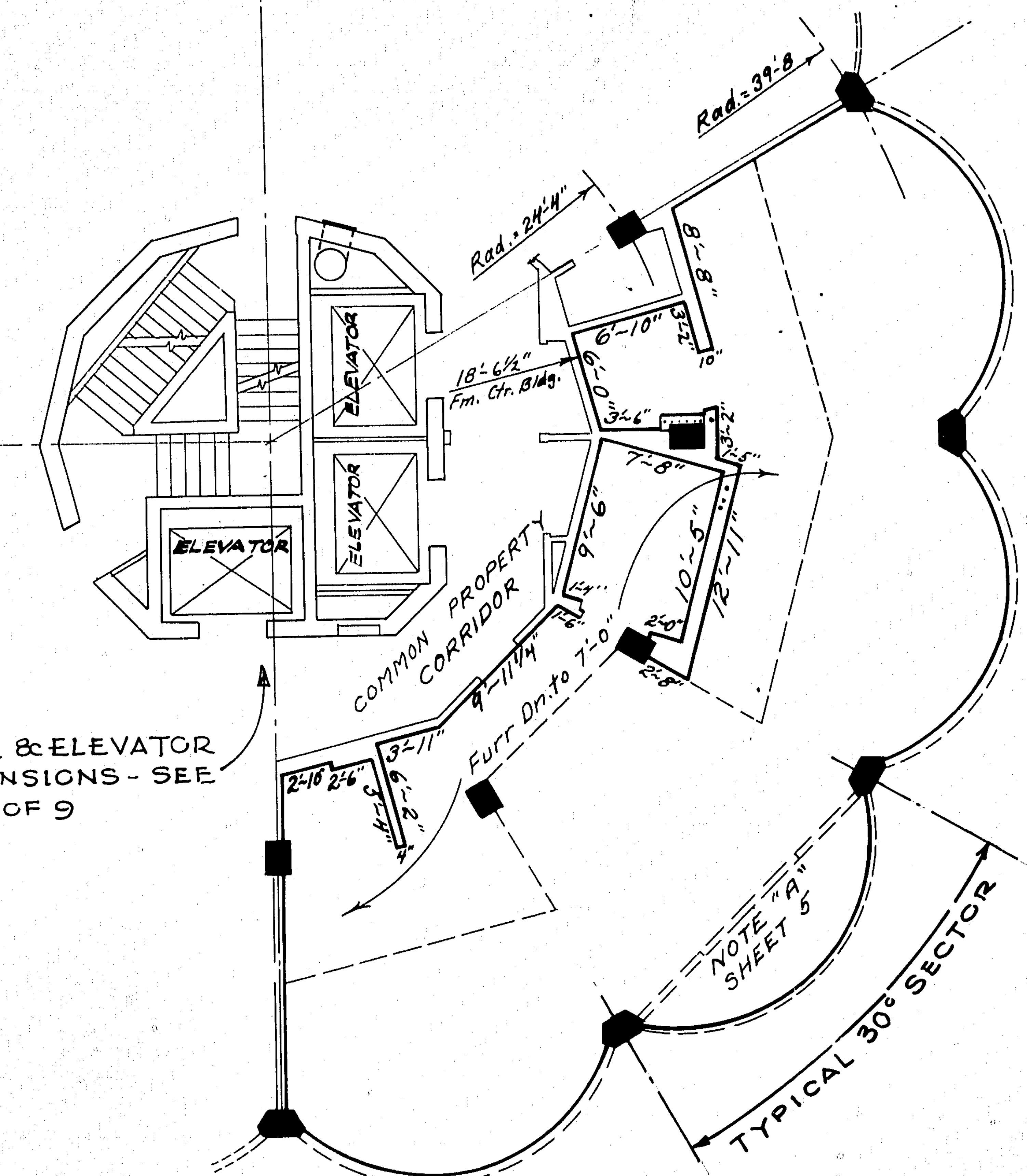
TYPE "B" Floors - 19 and 23 Scale - 1/8" = 1'-0"
