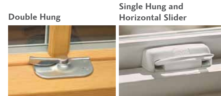
Cam Latch for Double Hung Includes Sash Handle and Thumb Lift Shown in Brushed Chrome
