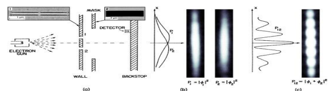
Figure 1. Simplified setup. (a) An electron beam passes through a wall with two slits in it. A movable mask is positioned to block the electrons, only allowing the ones traversing through slit 1 ( P_1 ), slit 2 ( P_2 ), or both ( P_{12} ) to reach the backstop and detector. (b), (c) Probability distributions are shown (experimental in false-color intensity) for electrons that pass through a single slit (b), or the double-slit (c). Inset 1, 2: electron micrographs of the double-slit and mask are shown. The individual slits are 62 nm wide \times 4 \mu m tall with a 150 nm support structure midway along its height, and separated by
