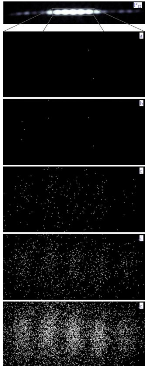
Figure 3. Buildup of electron diffraction. 'Blobs' indicate the locations of detected electrons. Shown are inter6+mediate build-up patterns from the central five orders of the diffraction
