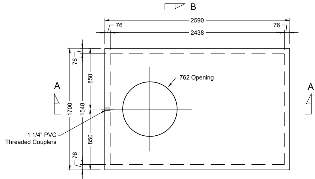
PLAN VIEW
