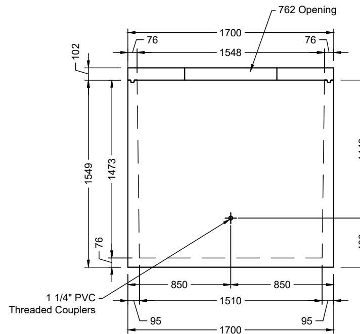
SECTION B-B
