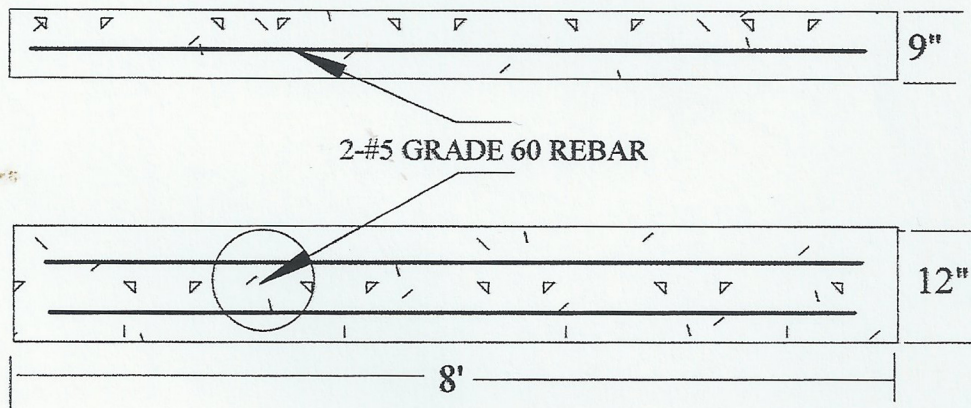
8'X12"X9" CONCRETE BASE BEAM
