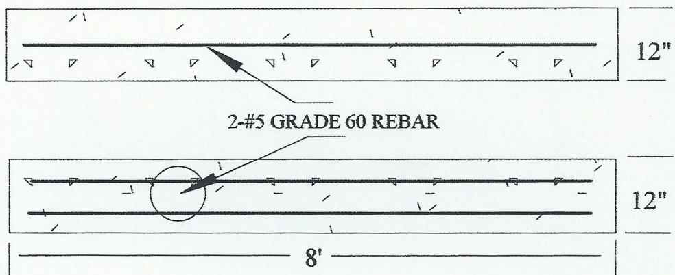
8'X12"X12" CONCRETE BASE BEAM
