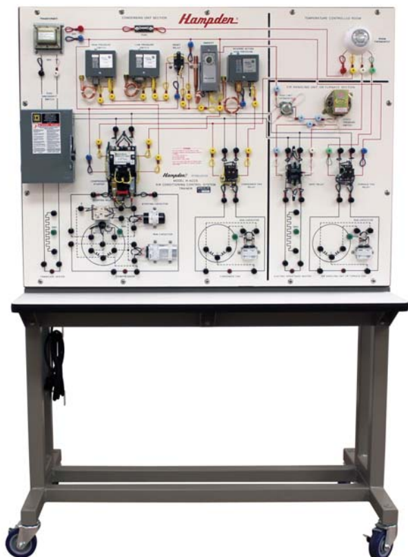
MODEL H-ACCS-1A Air Conditioning Control System Dimensions: 75"H x 48"W x 30"D Shipping Weight: 450 lbs
