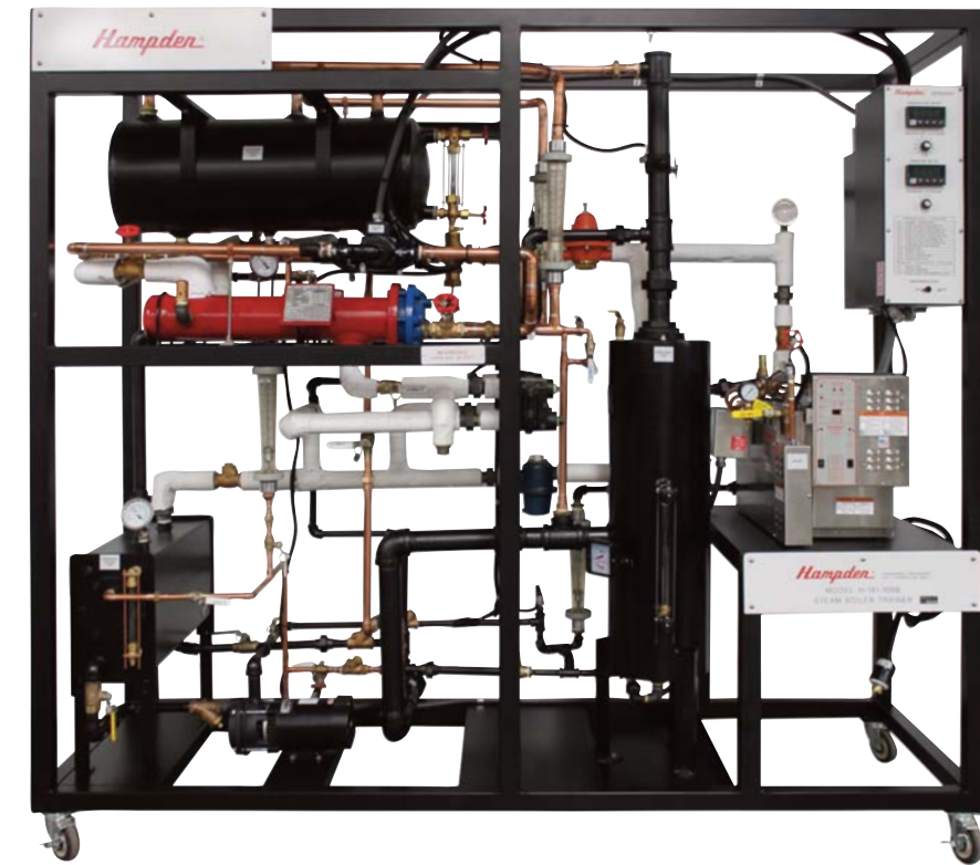
MODEL H-181-100B Steam Boiler Trainer
