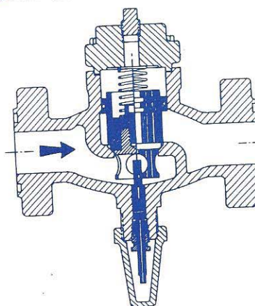
TYPE R PISTON TYPE CHECK VALVE
