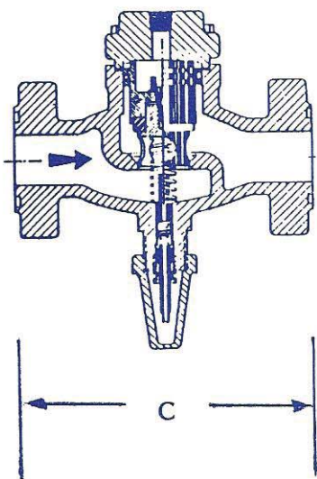
TYPE G GAS POWERED CHECK VALVE
