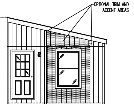
OPTIONAL FRONT ENDWALL WITH ACCENT AREAS
