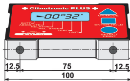
Right illustration: Left and lower side CLINOTRONIC PLUS with threaded holes M3x8/10 e.g. 015-PLUS-LG45
