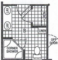
OPTION CORNER SHOWER BATH
