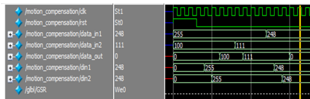
Figure 16: simulation results of motion compensation
