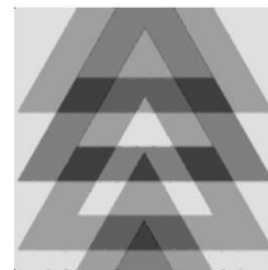
Figure 3. Output image
