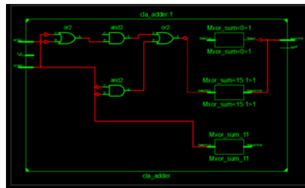
Figure 12: RTL Schematic internal block diagram of hidden layer.
