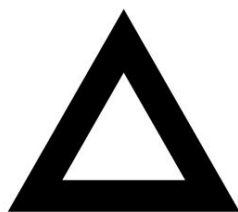
Figure 2: input image
