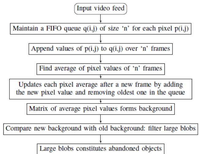
Figure 7: Proposed Flow chart.
