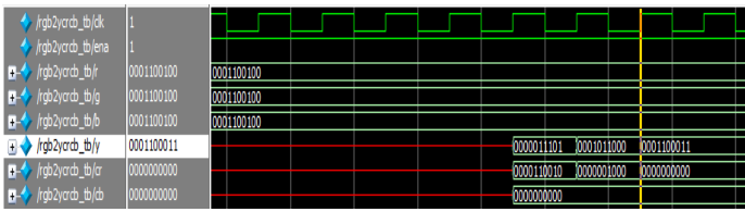
Figure 13: Simulation results for Conversion
