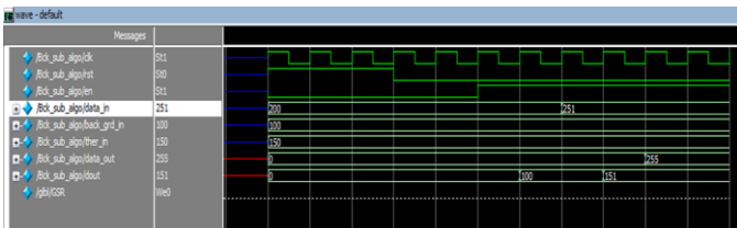
Figure 14: simulation results of background subtraction
