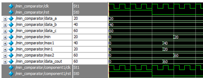
Figure 15: simulation results of closing filter
