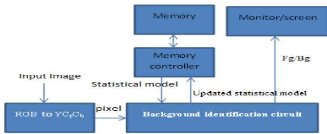
Figure 1. Block diagram for proposed GMM
