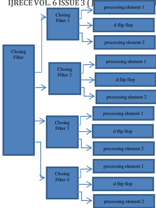
Figure 9: RTL Schematic block diagram of closing filter.
