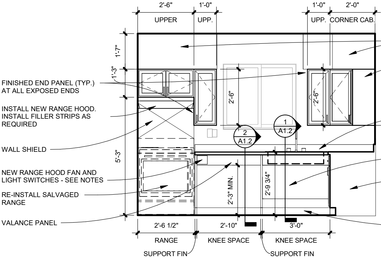
2-BED HC UNIT KITCHEN ELEVATION
