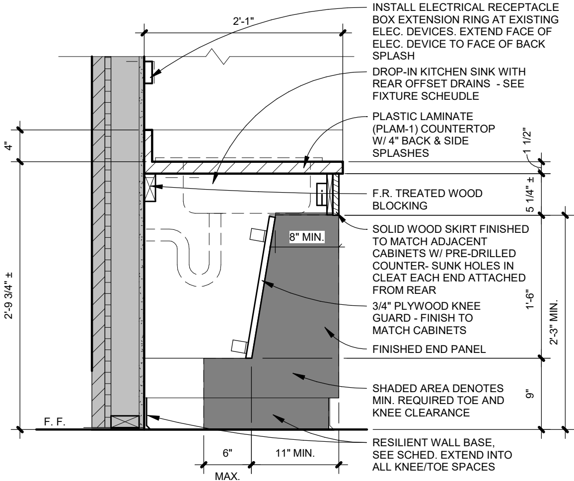
KITCHEN SINK DETAIL - ACCESSIBLE
