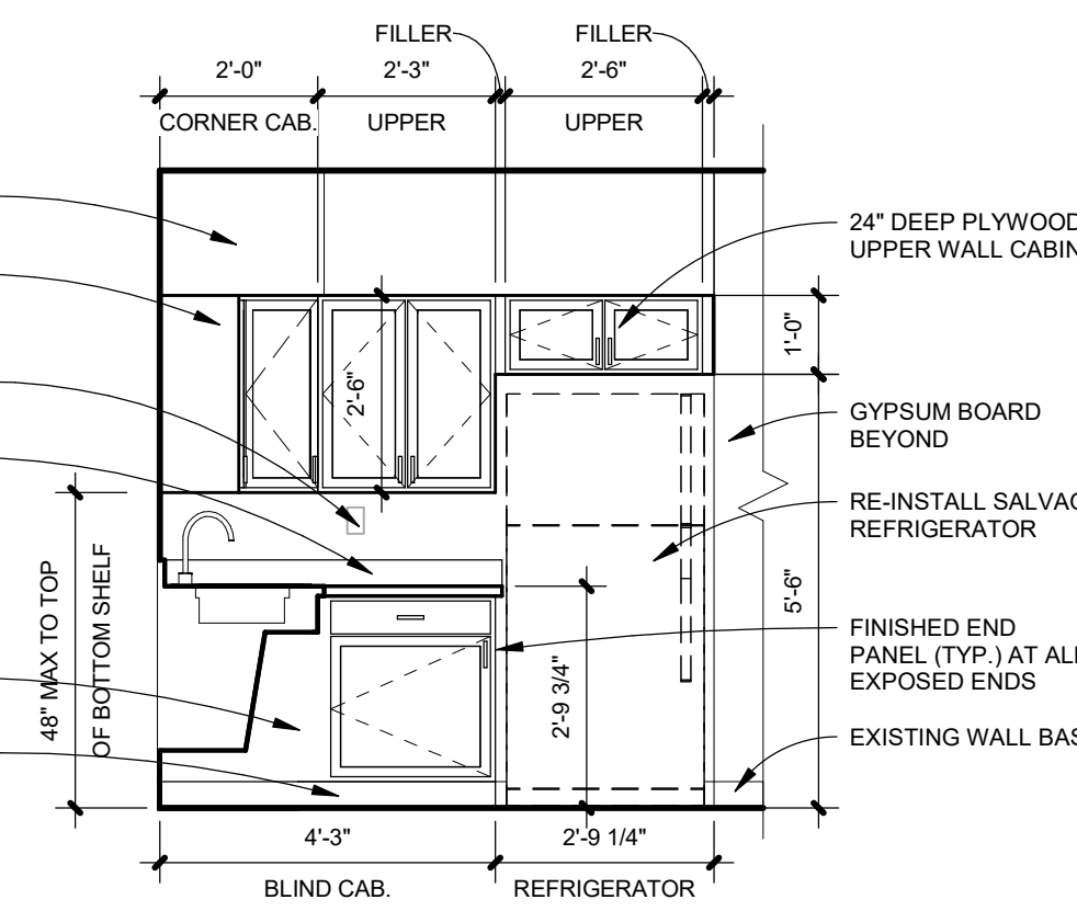
2-BED HC UNIT KITCHEN ELEVATION
