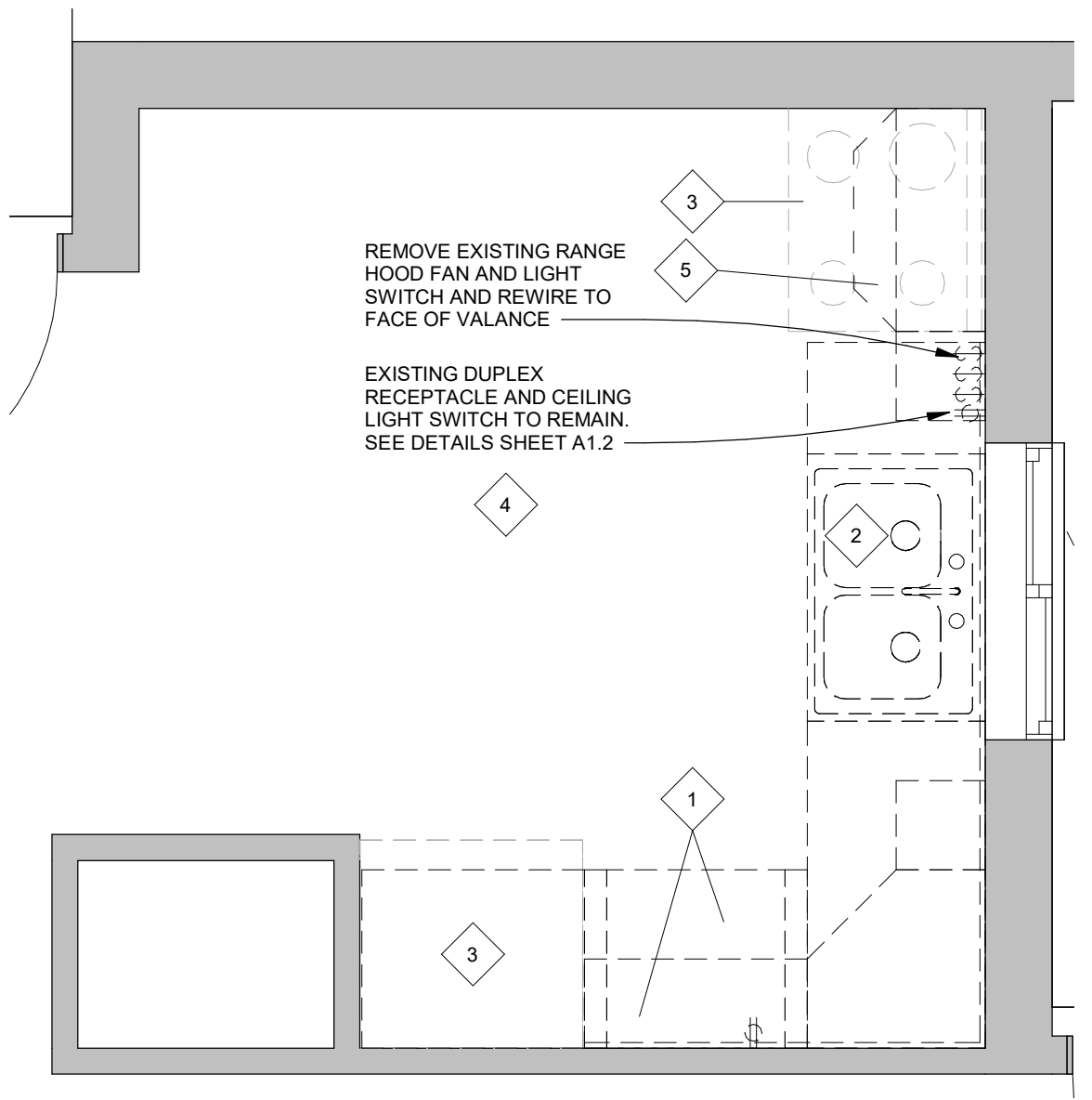
2-BED HC UNIT KITCHEN DEMO PLAN
