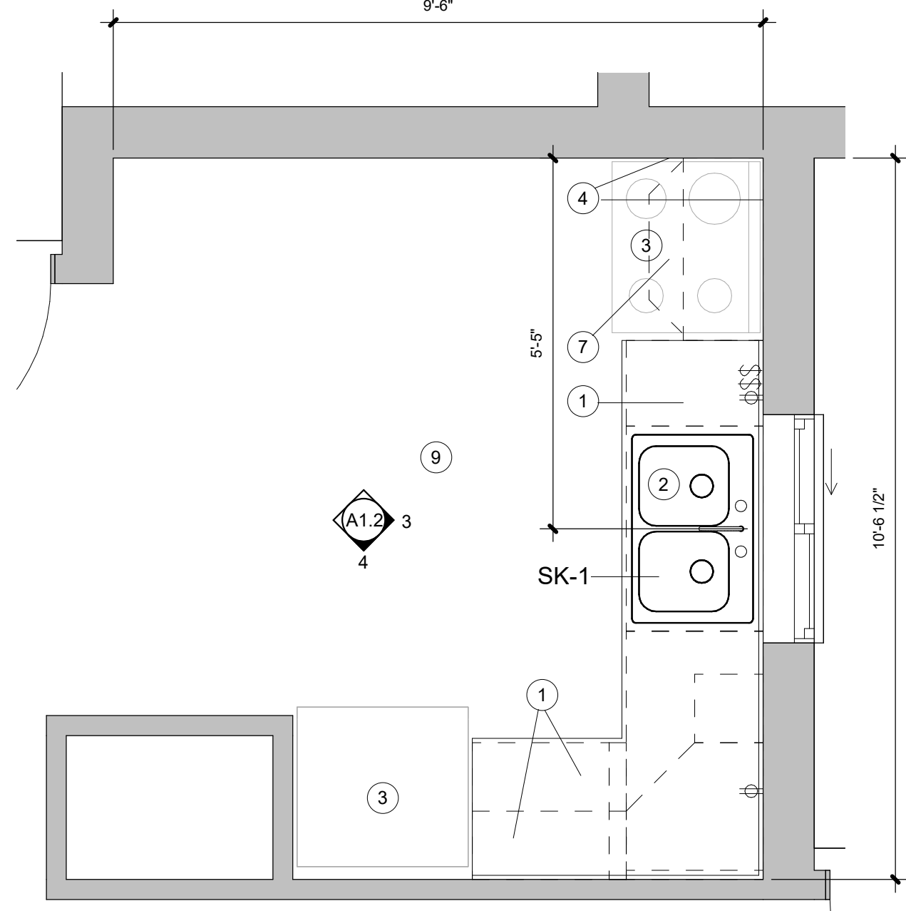
2-BED UNIT KITCHEN PLAN
