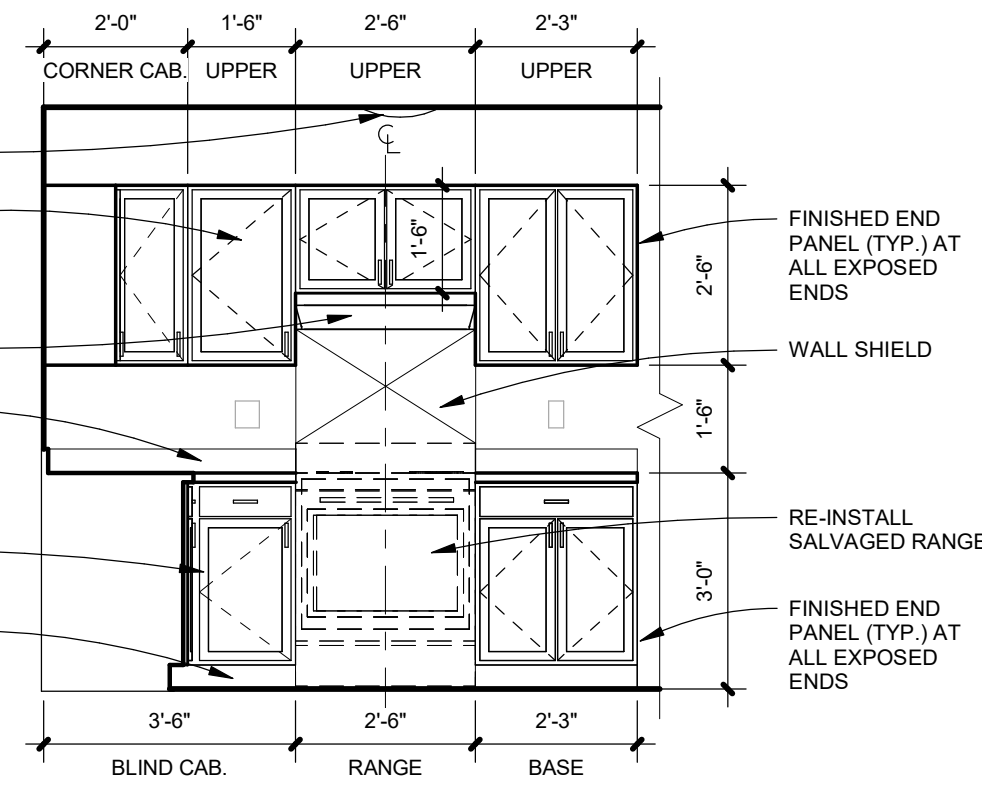
3-BED UNIT KITCHEN ELEVATION
