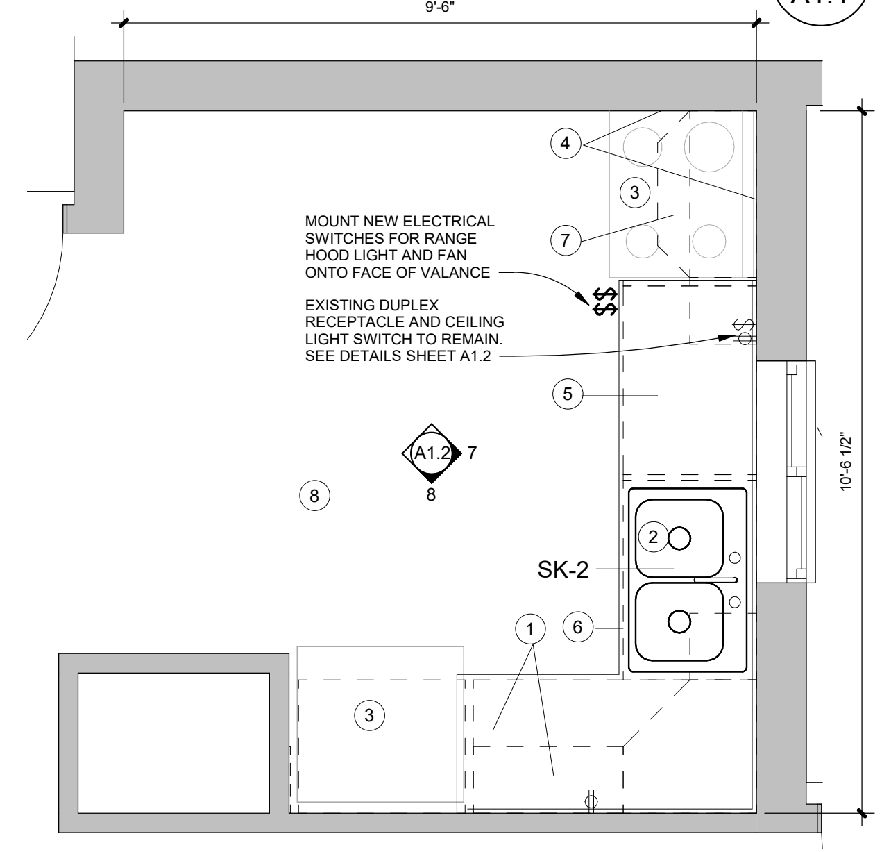
3-BED UNIT KITCHEN PLAN
