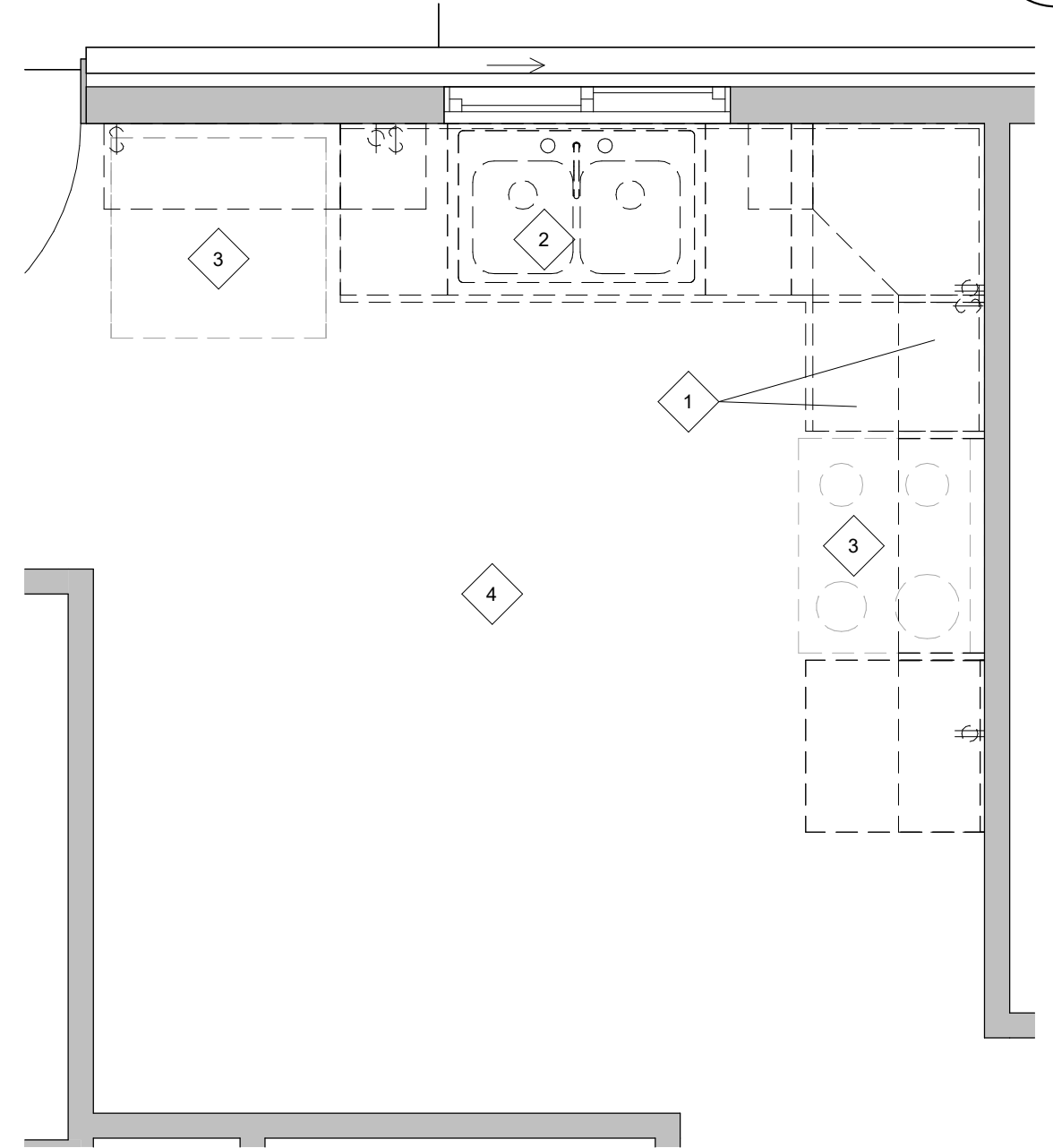
3-BED UNIT KITCHEN DEMO PLAN
