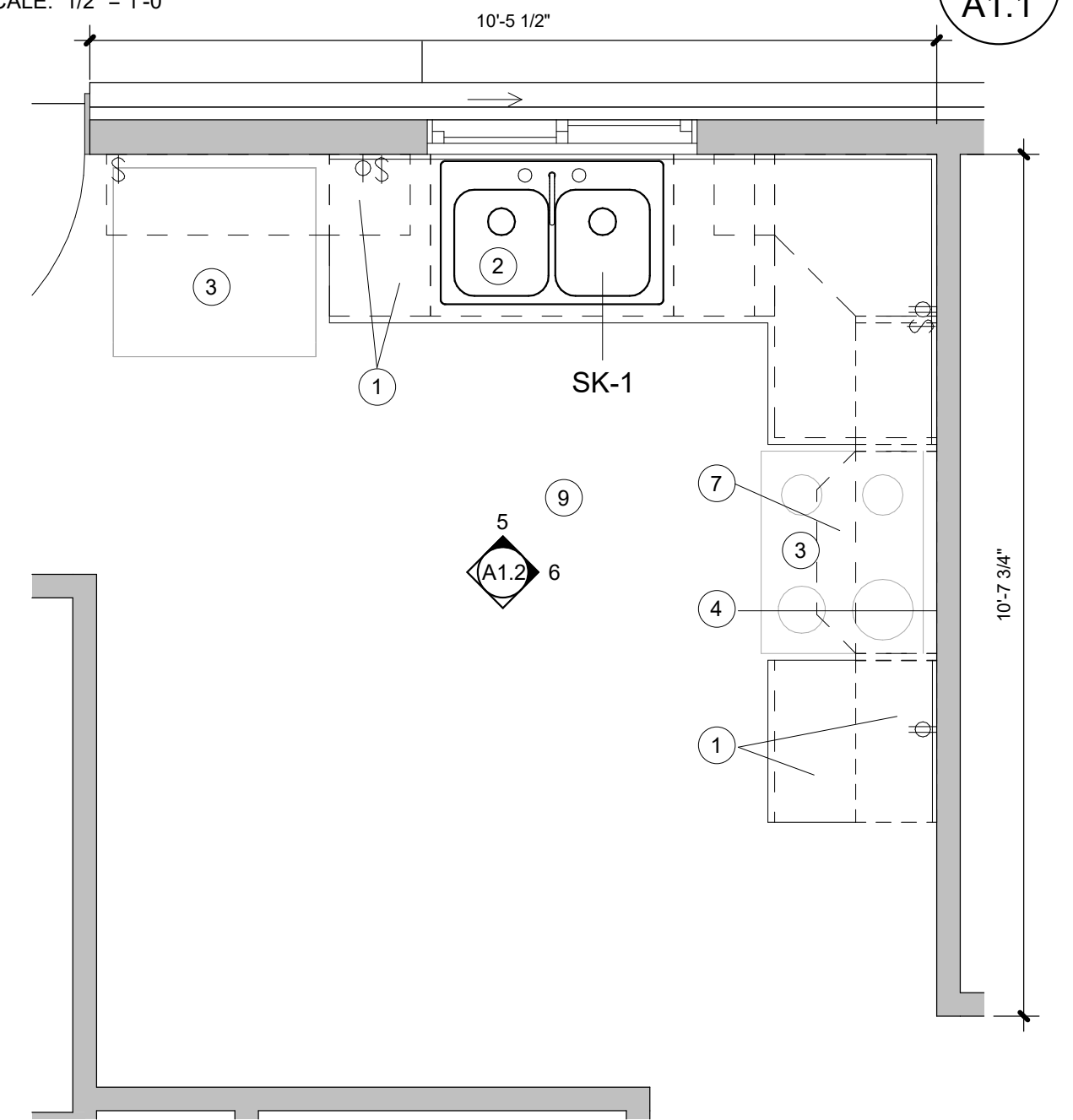
2-BED UNIT KITCHEN PLAN
