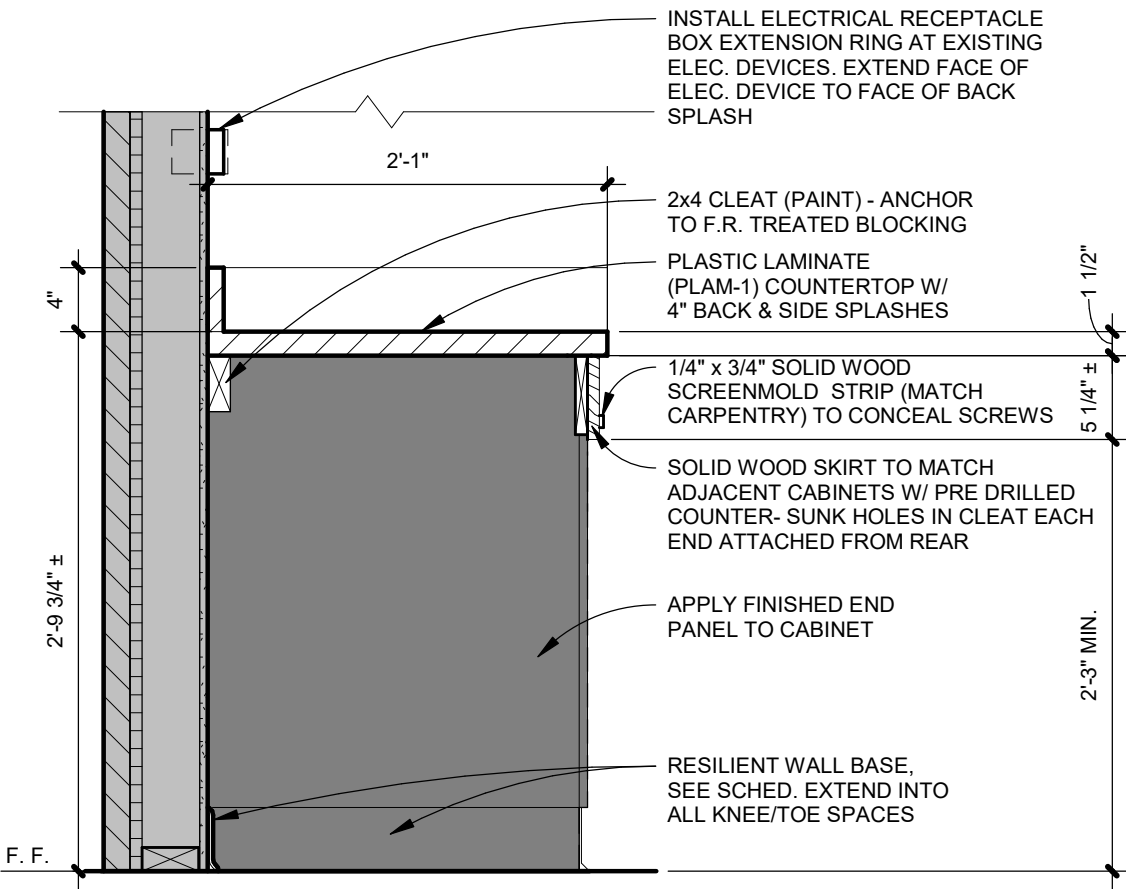
COUNTER DETAIL - ACCESSIBLE
