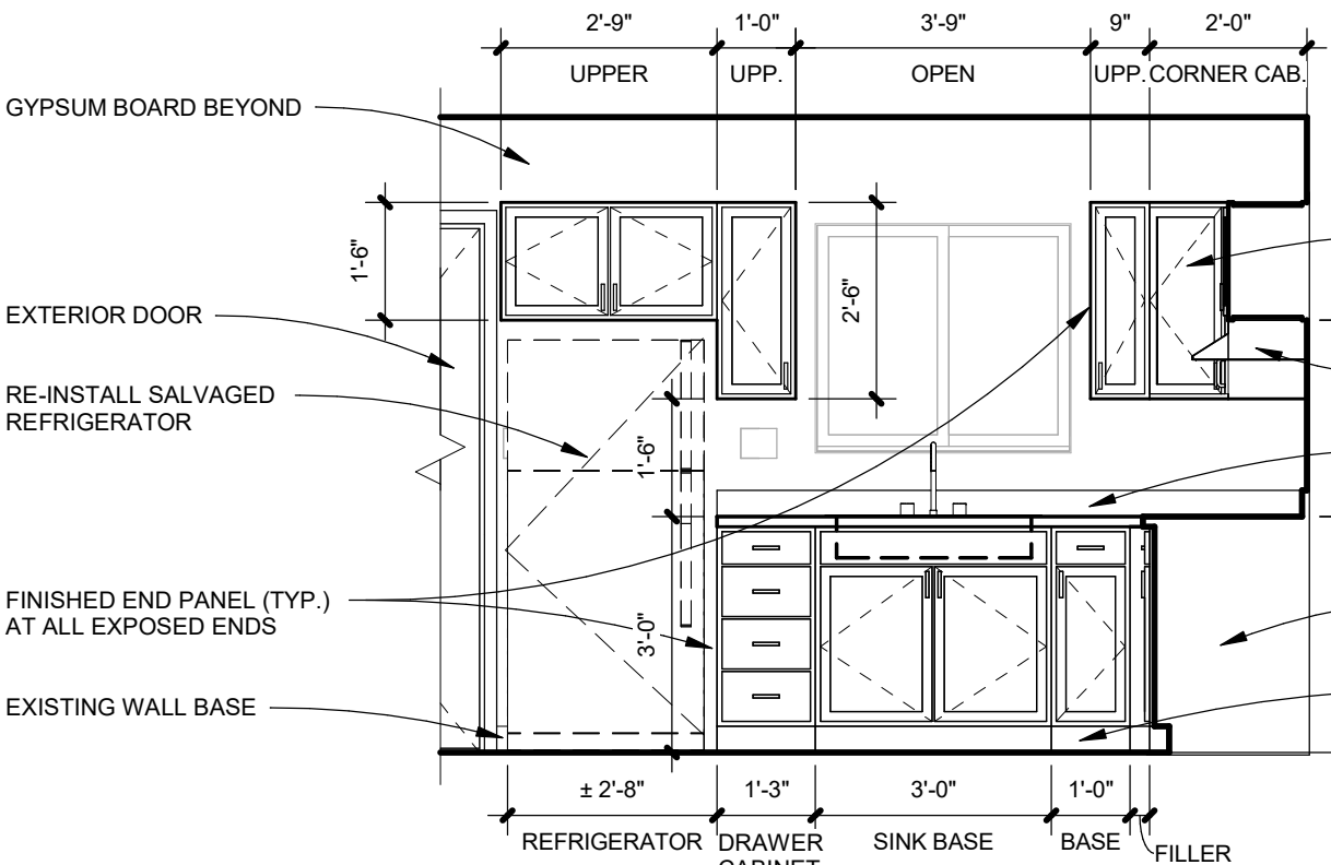
3-BED UNIT KITCHEN ELEVATION
