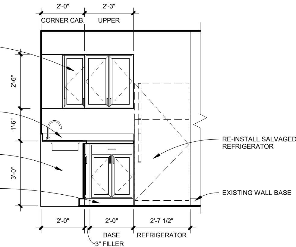
2-BED UNIT KITCHEN ELEVATION
