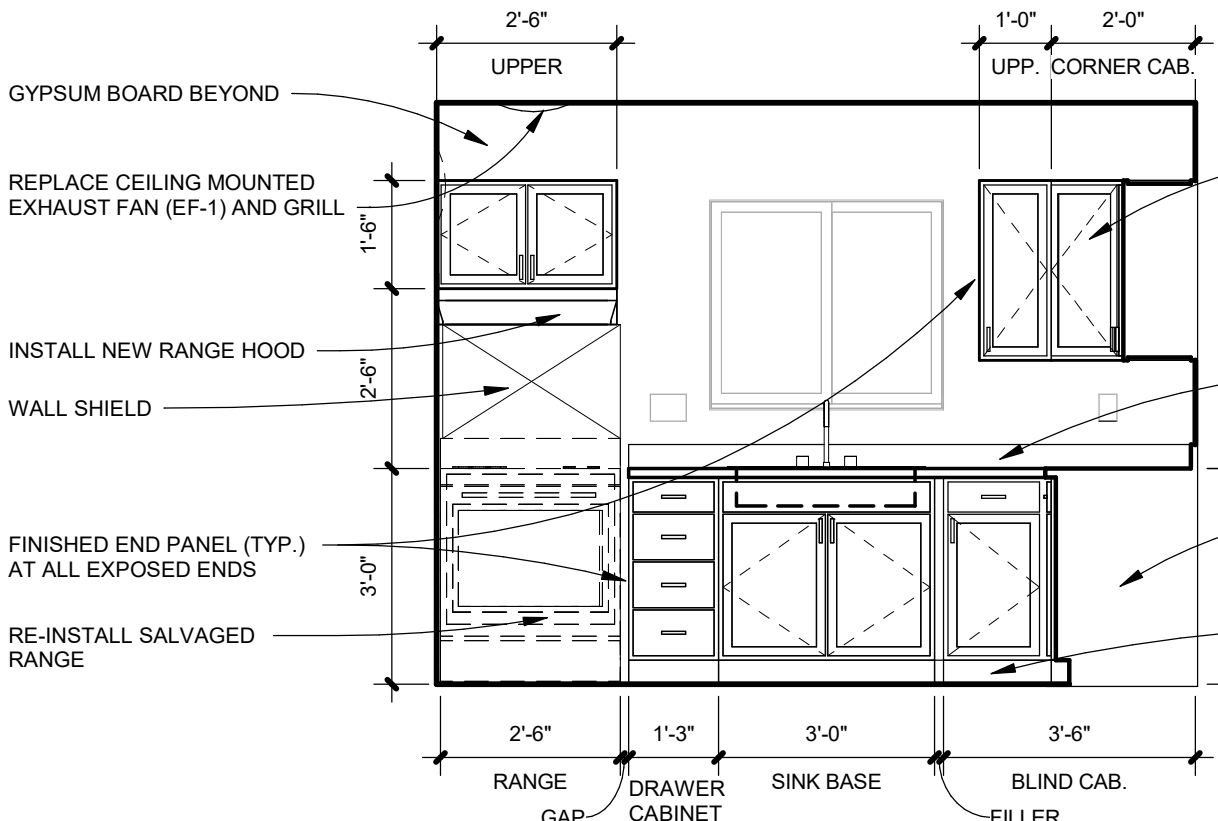
2-BED UNIT KITCHEN ELEVATION
