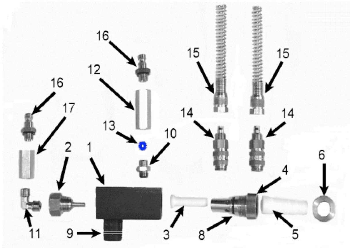
Illustration 1 Spareparts of the Injector
