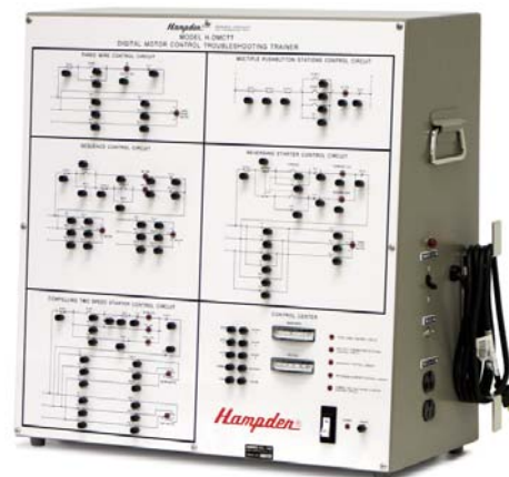
The Hampden MODEL H-DMCTT Digital Motor Control Troubleshooting Trainer Dimensions: 26"H x 24"W x 11"D Shipping Weight: 75 lbs.
