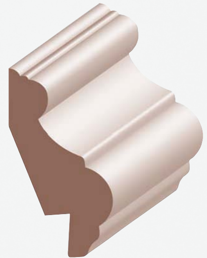
1-1/8 x 2 Panel Cap [with 1/2"- 5/8" Rab't] 615P Poplar N/S
