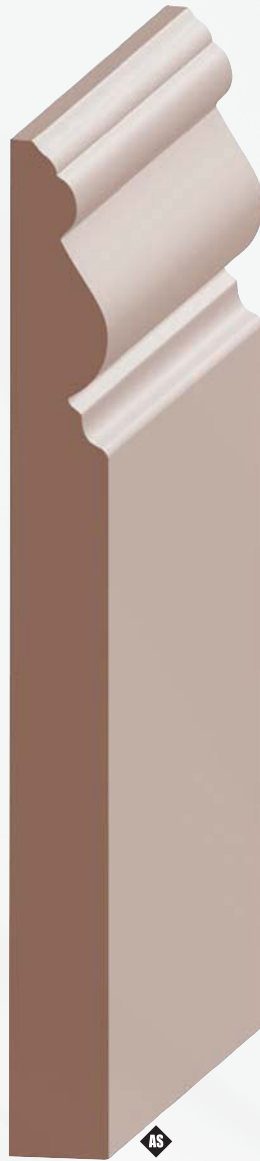
9/16 x 5-3/8 Santa Fe/#175 Base 338P-5 Poplar N/S 338-O5 Oak N 338ALD-5 Superior Alder N 338KA-5 Knotty Alder N 338C-5 Cherry N/S 338MH-5 Mahogany N/S 338MP-5 Maple N/S
