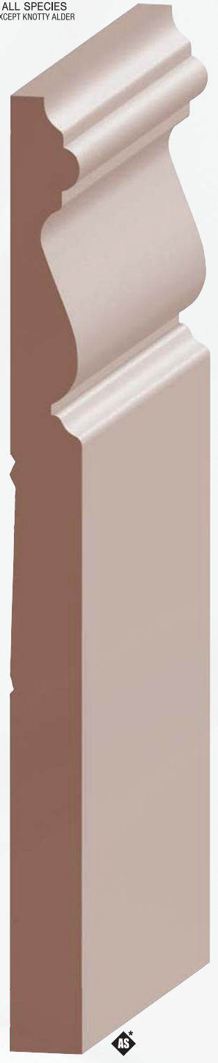
AS* 9/16 x 7-1/4 Monterey Base 361P-7 Poplar N/S 361-07 Oak N 361ALD-7 Superior Alder N/S 361C-7 Cherry N/S 361MH-7 Mahogany N/S 361MP-7 Maple N/S
