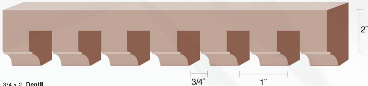
3/4 x 2 Dentil DE171P Poplar S DE171-O Oak S
