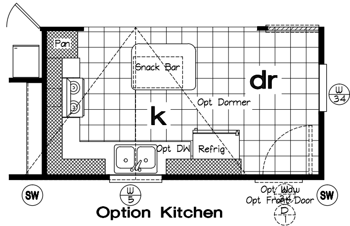
Golden Pacific - GP401P 2 Bedroom, Opt Study, Opt Porch - 787 Sq. Ft.
