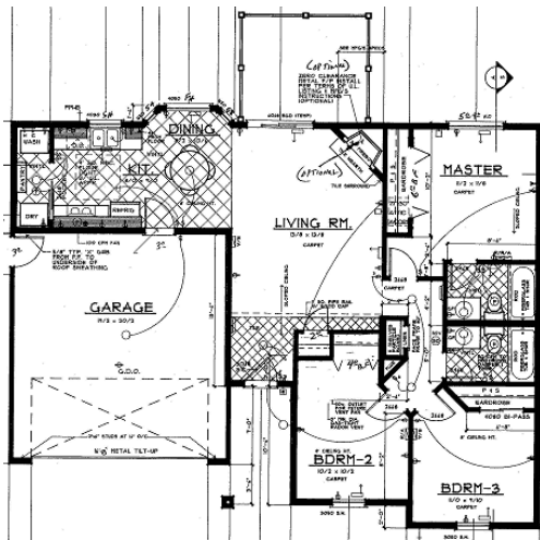
Chena Model 1,135 Finished Sq.Ft. 1-Car Garage
