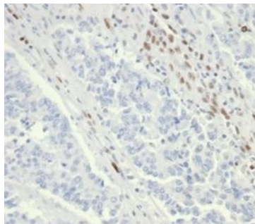
FFPE human colon stained with anti-MSH6 using DAB
