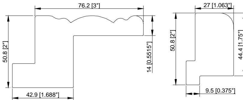
Tilt Out Z Frame
