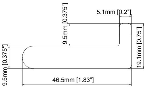
1.83" Sill plate with 3/8" light block (For 2.5" Mission Deco frame)
