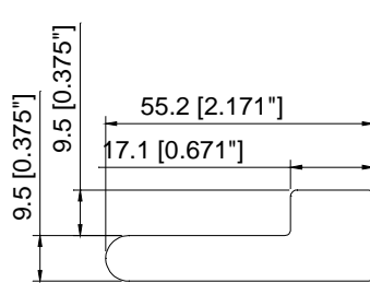
2.17" Sill with 3/8" Light block (L/Z)
