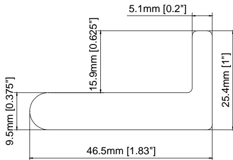
1.83" Sill plate with 5/8" light block (For 2.5" Mission Deco frame)
