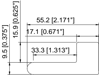
2.17" Sill with 5/8" Light block (L/Z)
