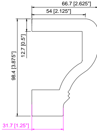
Designer Sill Cap(L)
