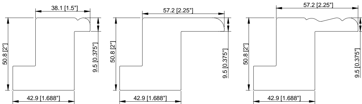
1 1/2" Beaded Z Frame
