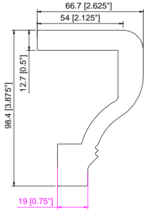
Designer Sill Cap(D/HS)
