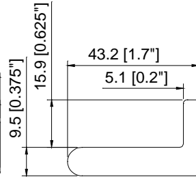
1.7" Sill with 5/8" Light block (Deco)
