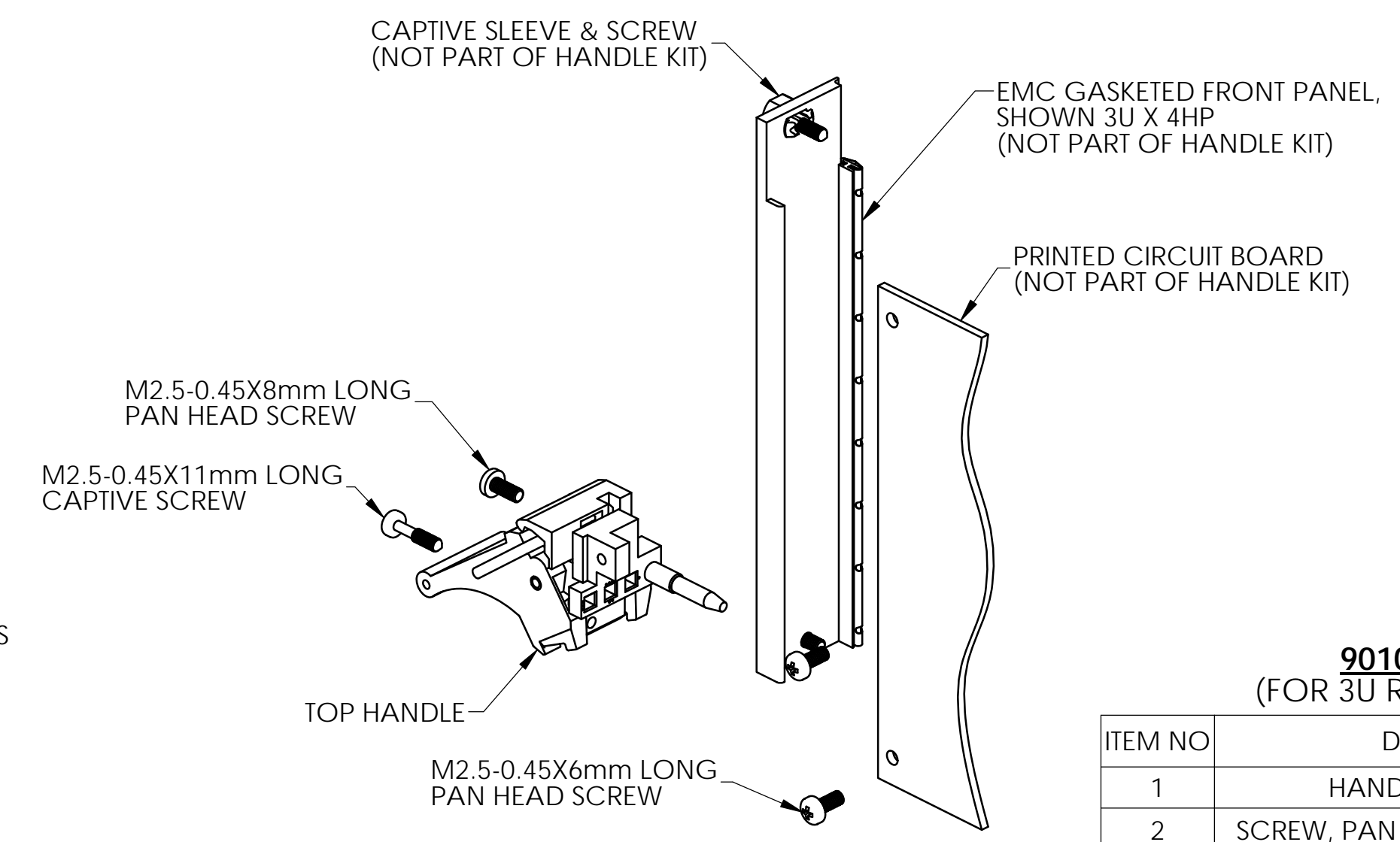
EXPLODED VIEW 3U RTM PLUG-IN CARD ASSEMBLY
