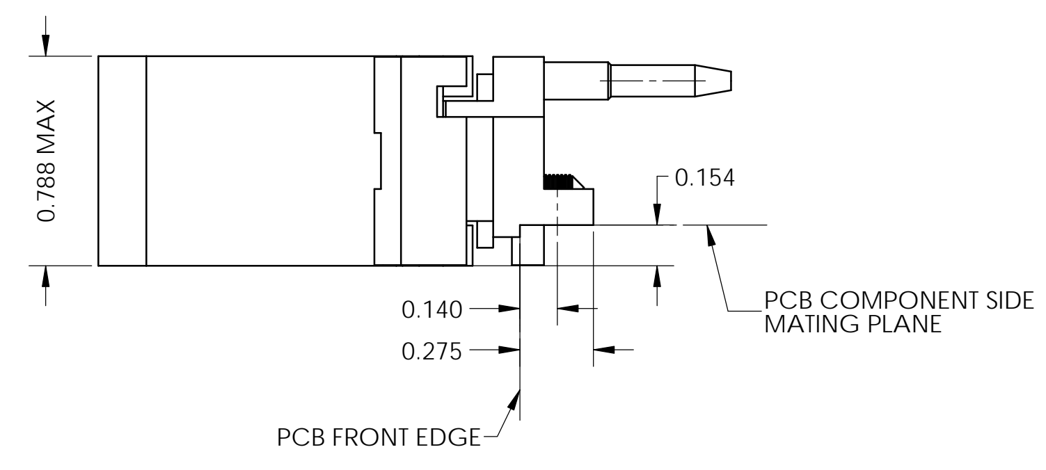
TOP HANDLE DETAIL
