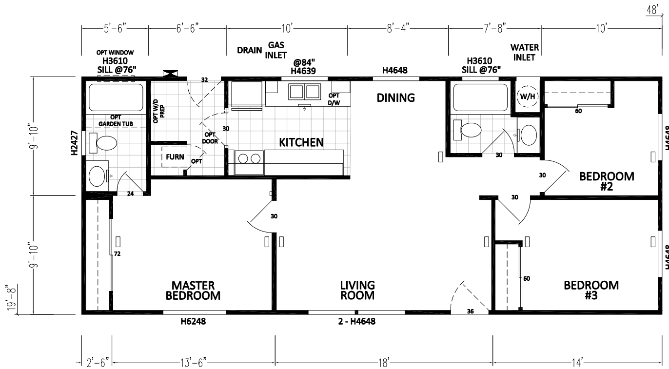
4617CTC 3BD - 2BA 4820 (944 SQ. FT. LIVING)
