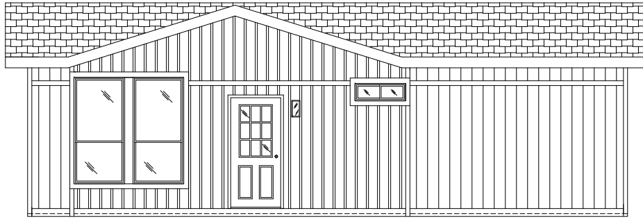
FRONT SIDEWALL W/ DORMER
