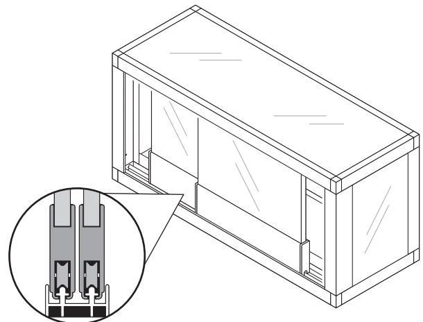
12. Install doors
