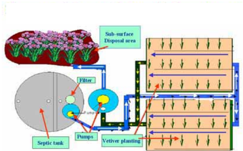
Figure 5: Layout of a domestic disposal system
