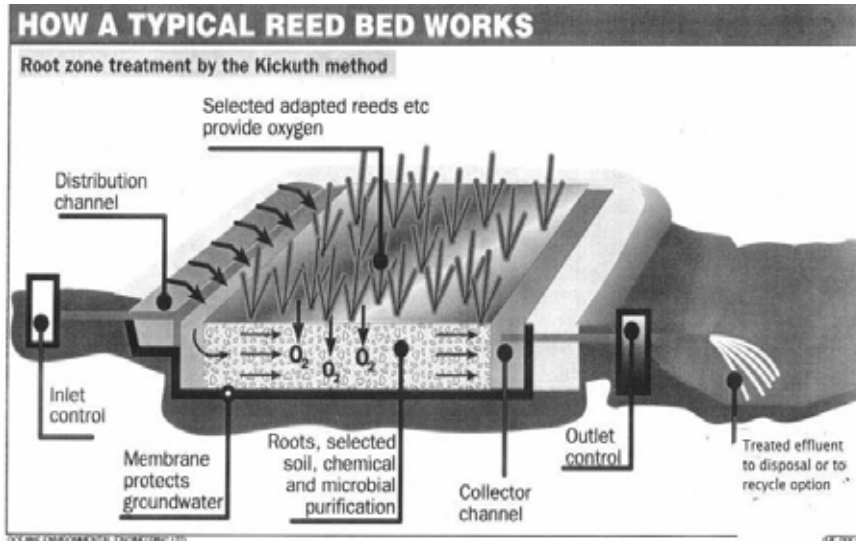
Figure 6: Workings of a typical reed bed
