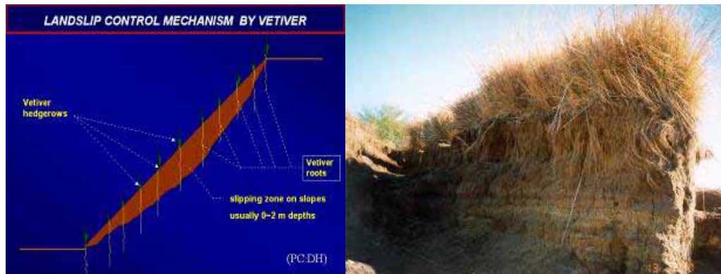
Figure 1: Left: Principles of slope stabilisation by Vetiver; right: Vetiver roots reinforcing this dam wall kept it from being washed away by flood
