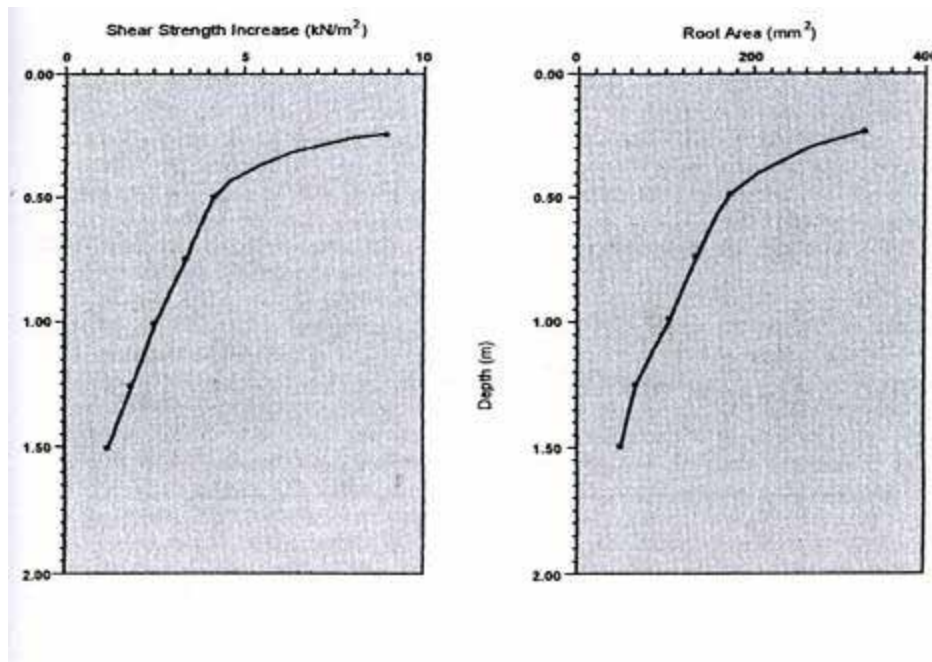
Figure 3: Shear strength of Vetiver root
