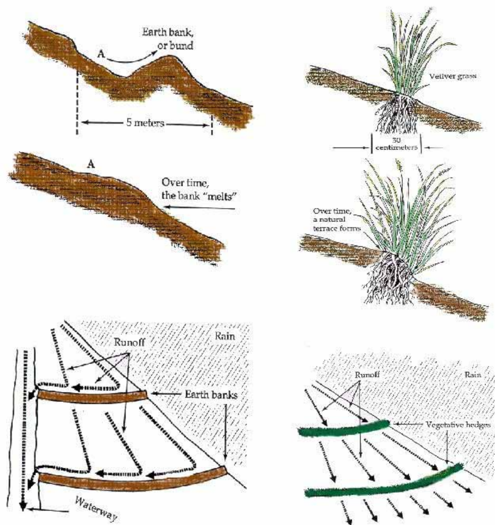
Figure 1: Above left: contour bank; below left: banks divert the water; above right: Vetiver grasses create banks or terraces over time; below right: Vetiver grasses slow the runoff to increase infiltration, and the water remains in the field (Greenfield 1989)
