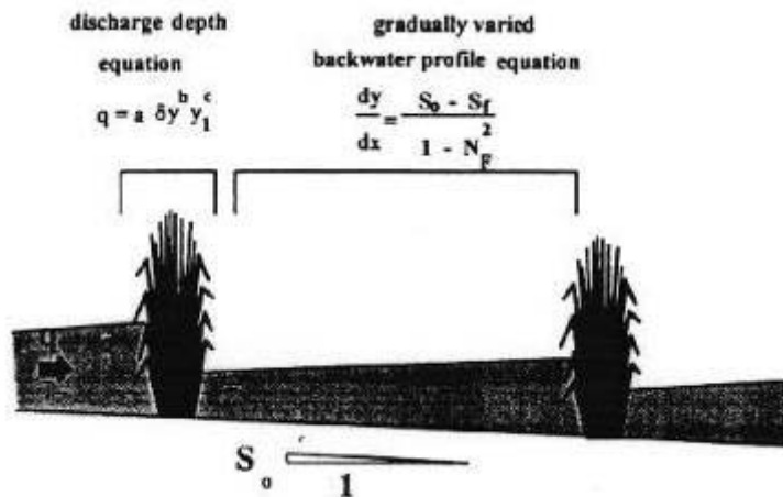
Figure 4: Hydraulic model of flooding through Vetiver hedges
