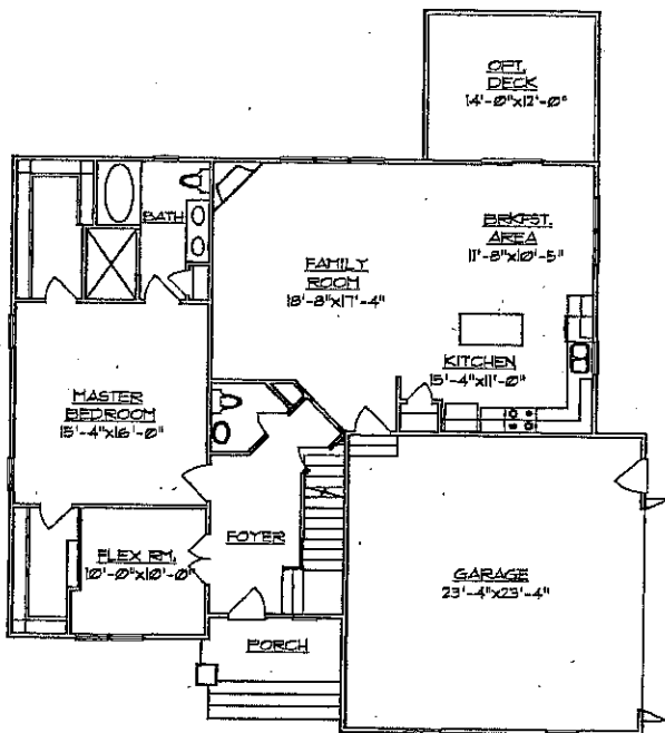
FIRST FLOOR PLAN 1449 SQ. FT. (HEATED) 564 SQ. FT. (GARAGE)
