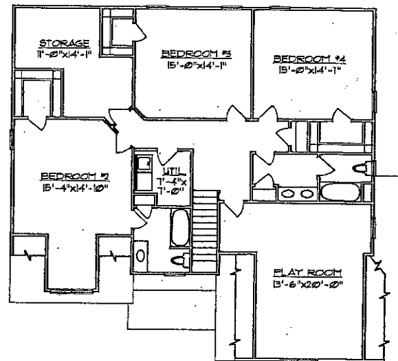
SECOND FLOOR PLAN 1408 SQ. FT. (HEATED) 325 SQ. FT. PLAYROOM (HEATED)
