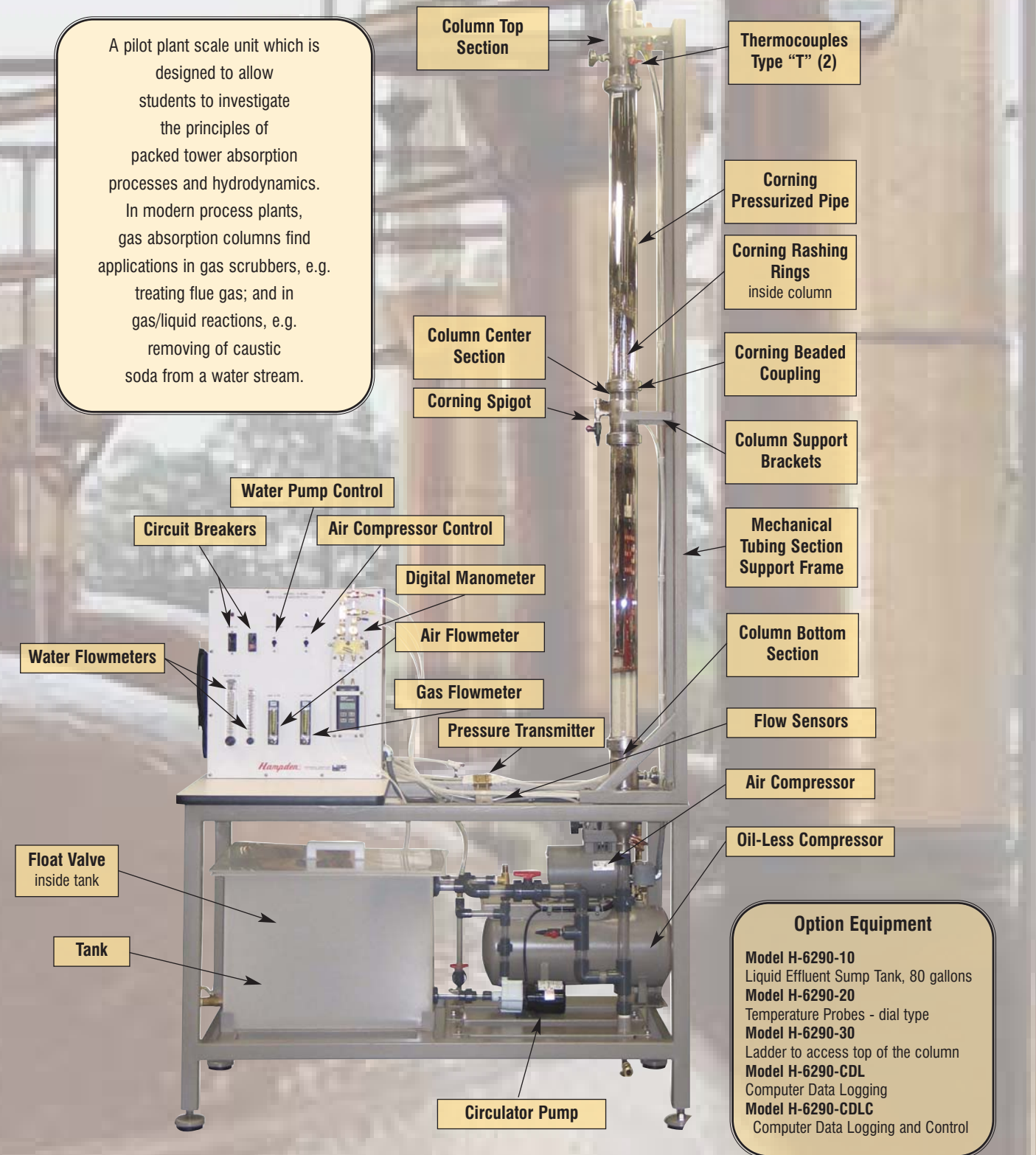
Hampden's Model H-6290 Gas/Liquid Absorption Column
