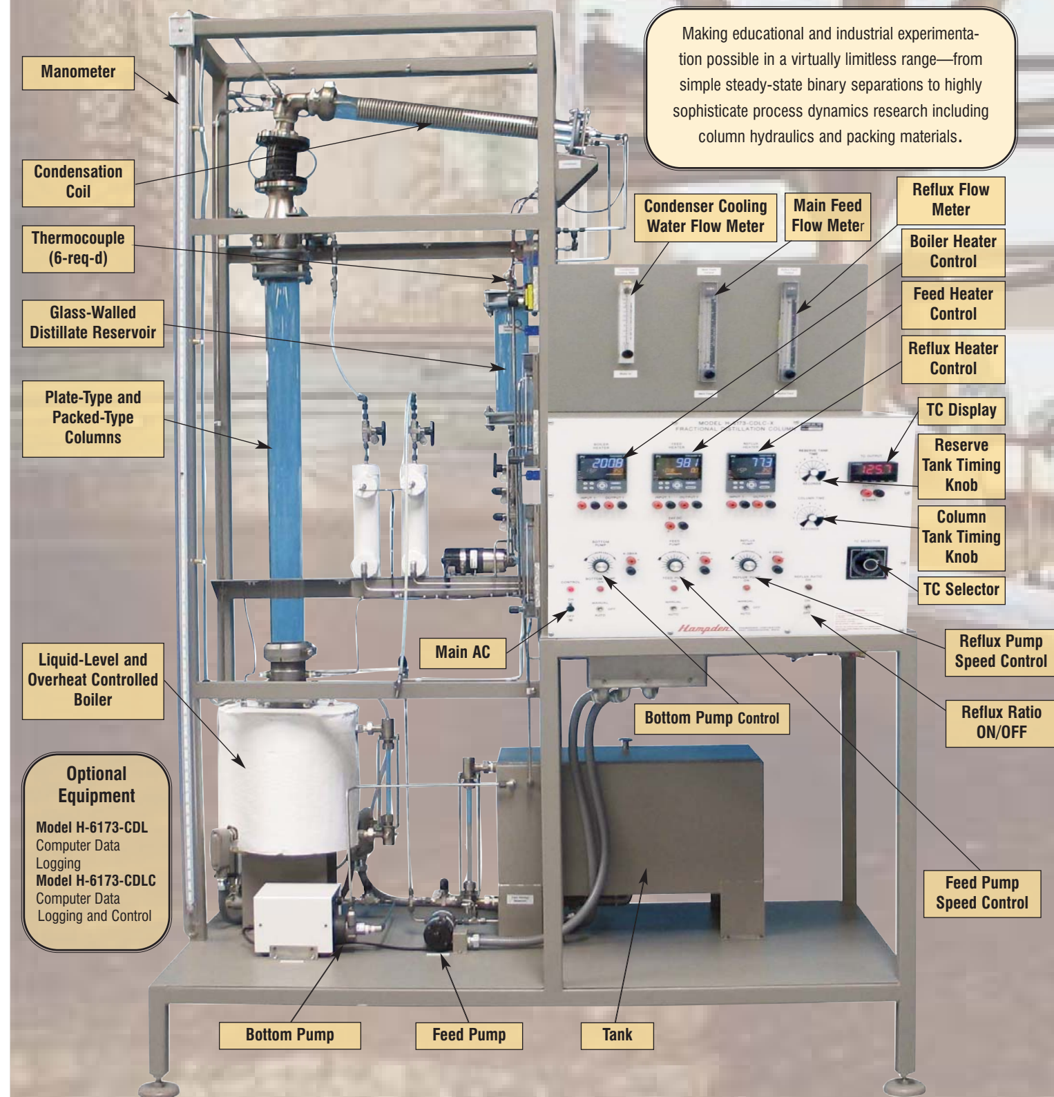
Hampden's Model H-6173 Continuous/Fractional Distillation System
