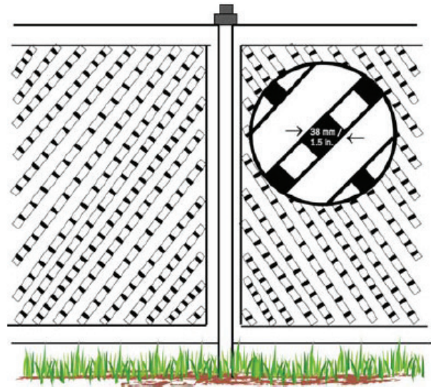
Recommended wood lattice opening
