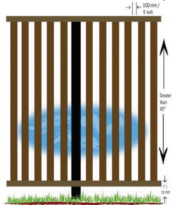
Recommended vertical bar spacing if horizontal bars are greater than 114.3cm (45 in) apart
