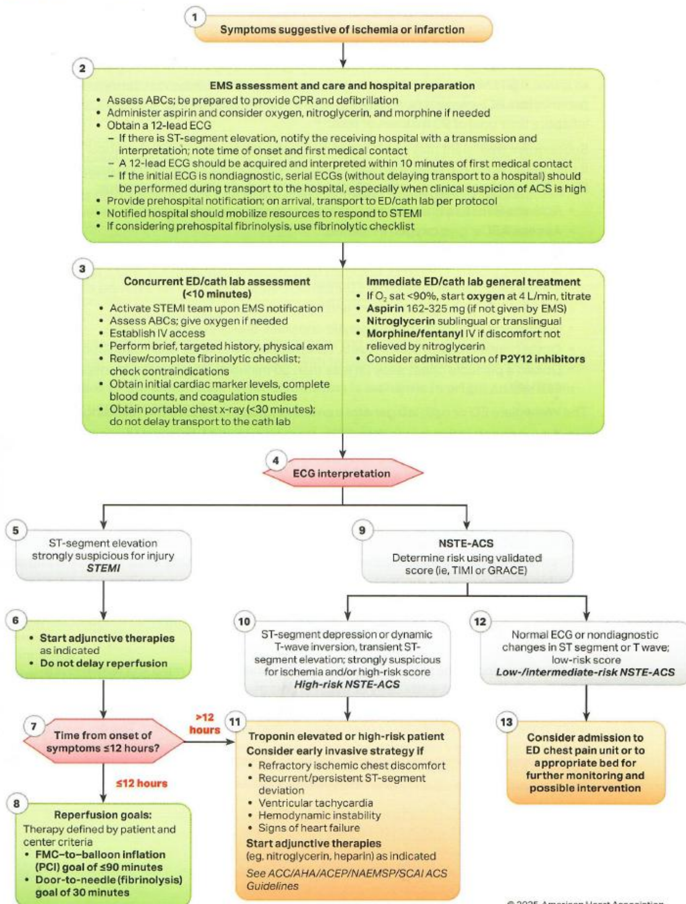
Figure 17. ACS Algorithm.
