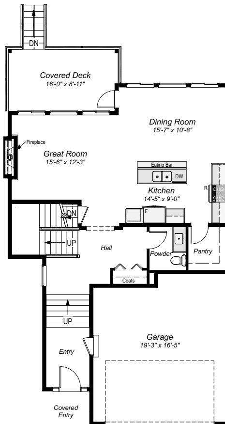
MAIN FLOOR PLAN 961 sq ft
